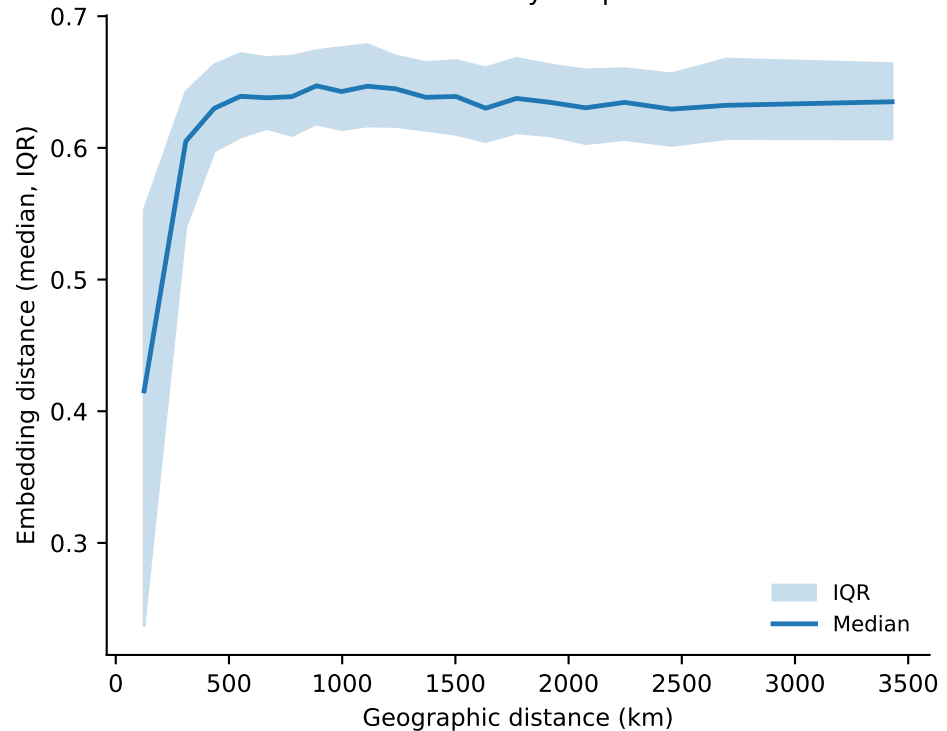
Binned median by km percentile
