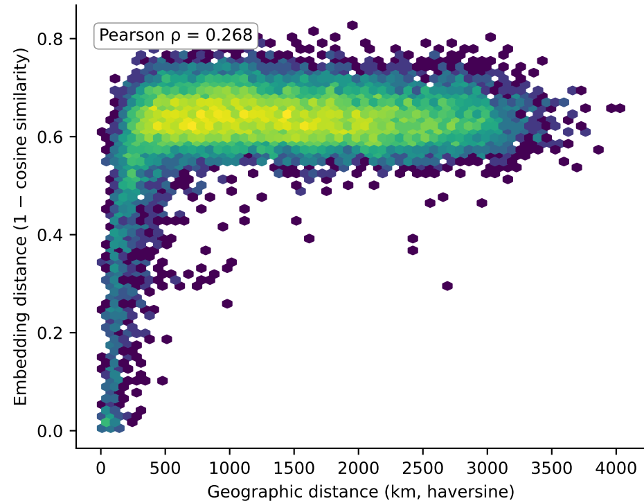
Pair-wise: embedding vs km (n=14992)
