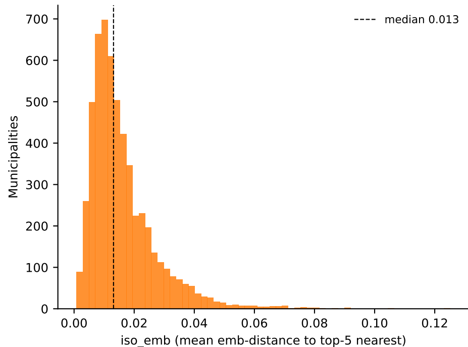
Network-revealed isolation
