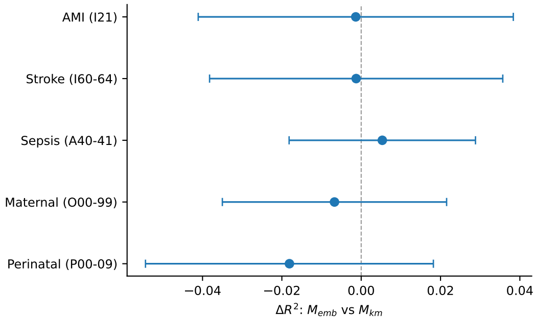
Embedding alone vs km alone
