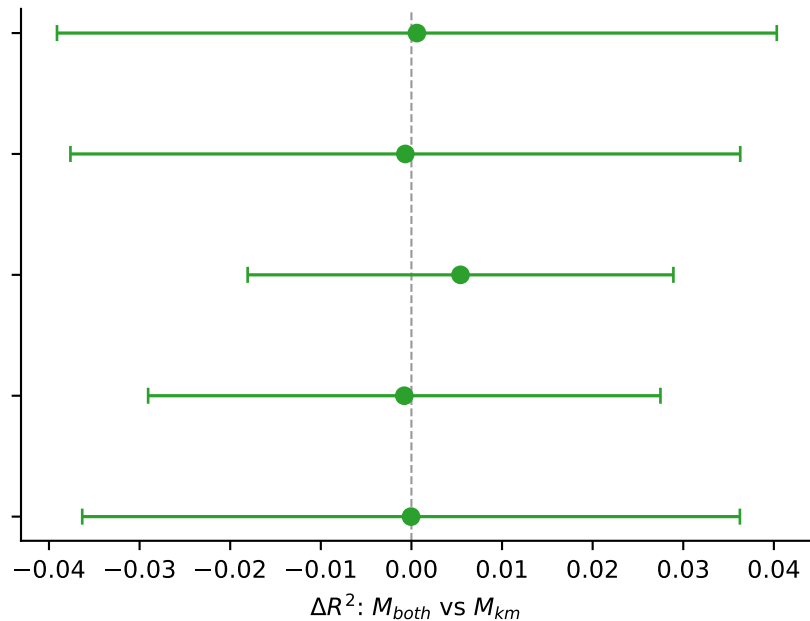
Embedding incremental gain over km
