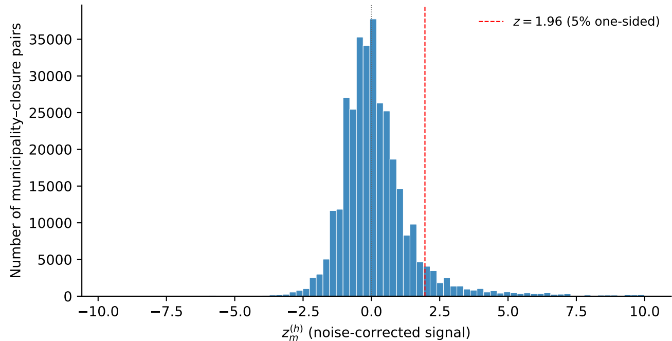
Distribution of perturbation z-signals (truncated at |z| < 10 for visibility)
