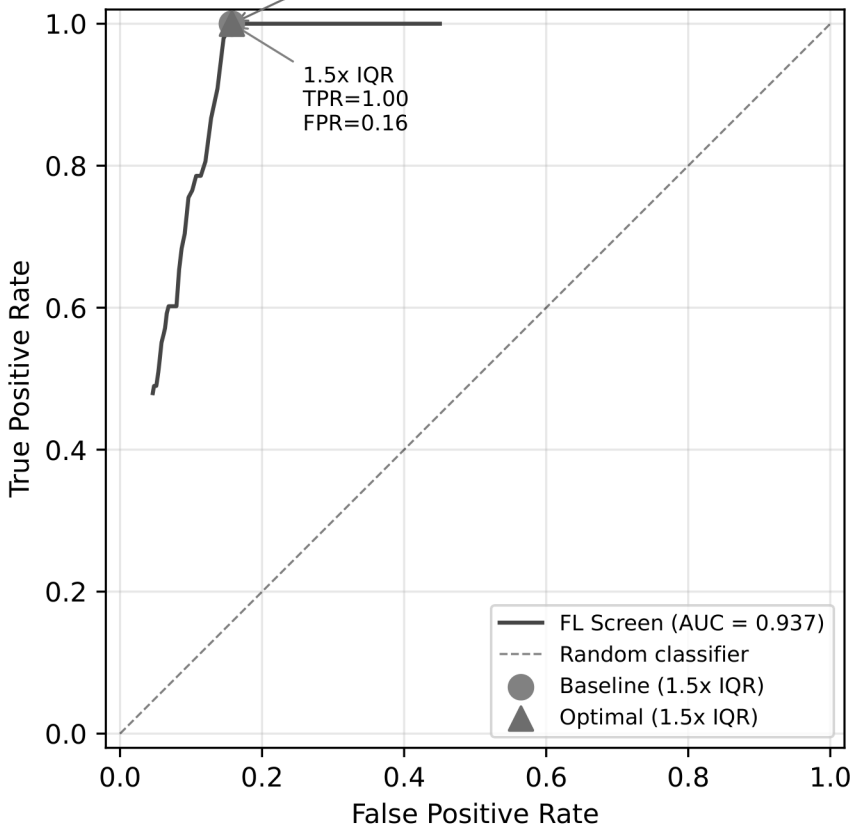
ROC Curve: FL Screen vs. CADE Ground Truth
