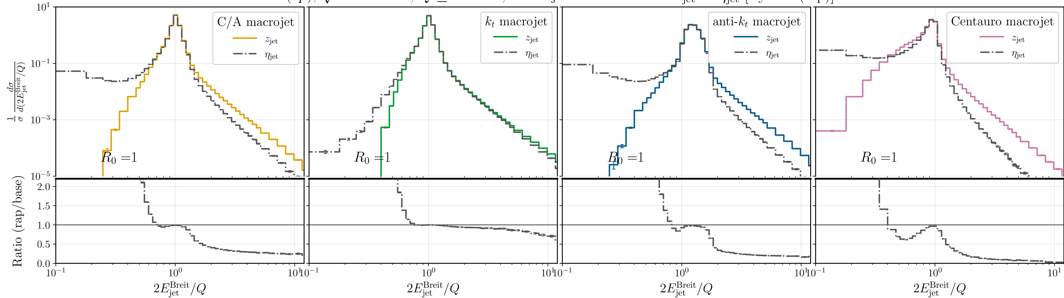
NC DIS ( ep ), \sqrt{s}=300 GeV, Q \geq 12 GeV, Macrojet reconstruction: z_{\text{jet}} vs \eta_{\text{jet}} [Pythia8(dip)]
