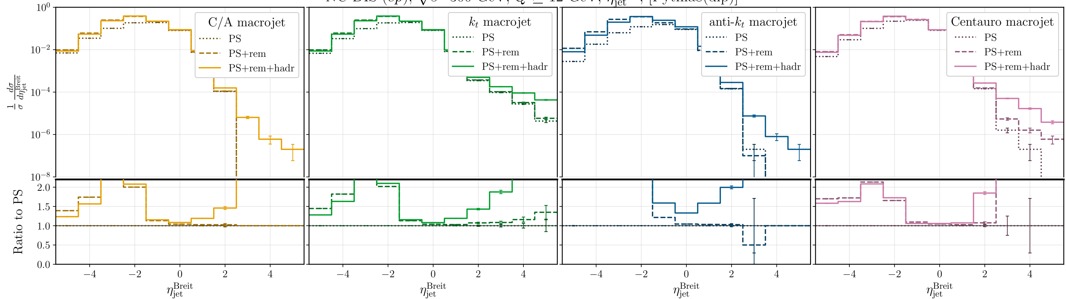
NC DIS ( ep ), \sqrt{s}=300 GeV, Q \geq 12 GeV, \eta_{\text{jet}}^{\text{Breit}} , [Pythia8(dip)]
