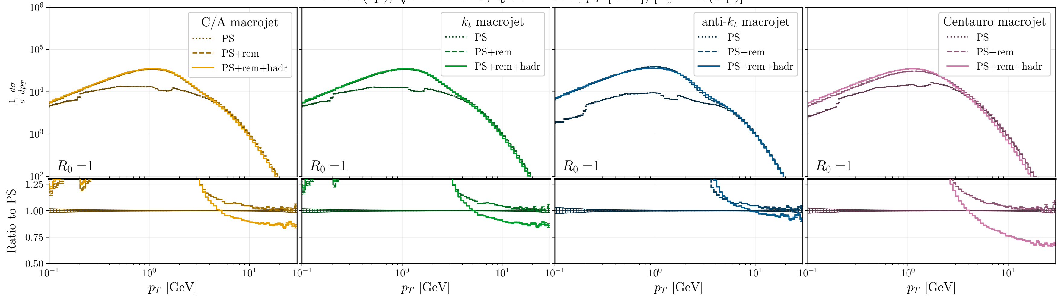
NC DIS ( ep ), \sqrt{s}=300 GeV, Q \geq 12 GeV, p_T [GeV], [Pythia8(dip)]
