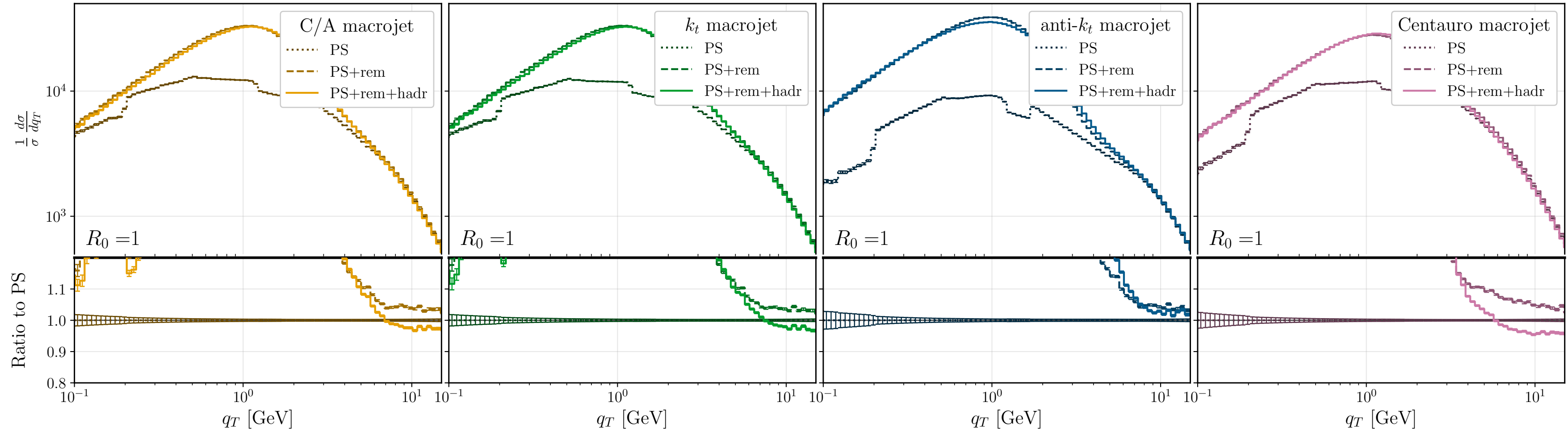
NC DIS ( ep ), \sqrt{s}=300 GeV, Q \geq 12 GeV, q_T [GeV], [Pythia8(dip)]
