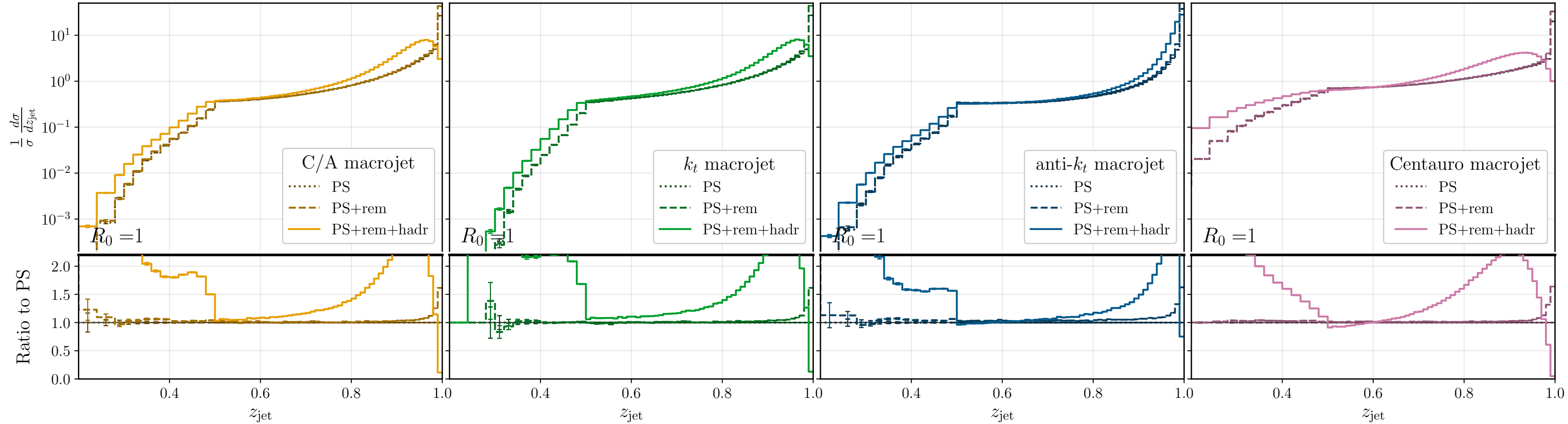
NC DIS ( ep ), \sqrt{s}=300 GeV, Q \geq 12 GeV, z_{\text{jet}} , [Pythia8(dip)]
