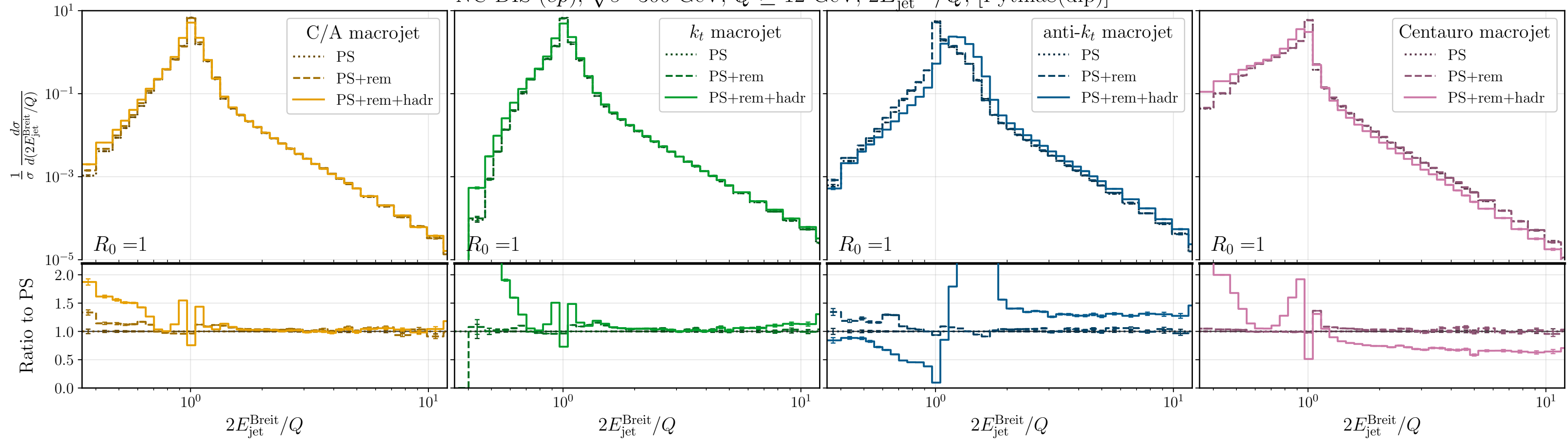
NC DIS ( ep ), \sqrt{s}=300 GeV, Q \geq 12 GeV, 2E_{\text{jet}}^{\text{Breit}}/Q , [Pythia8(dip)]
