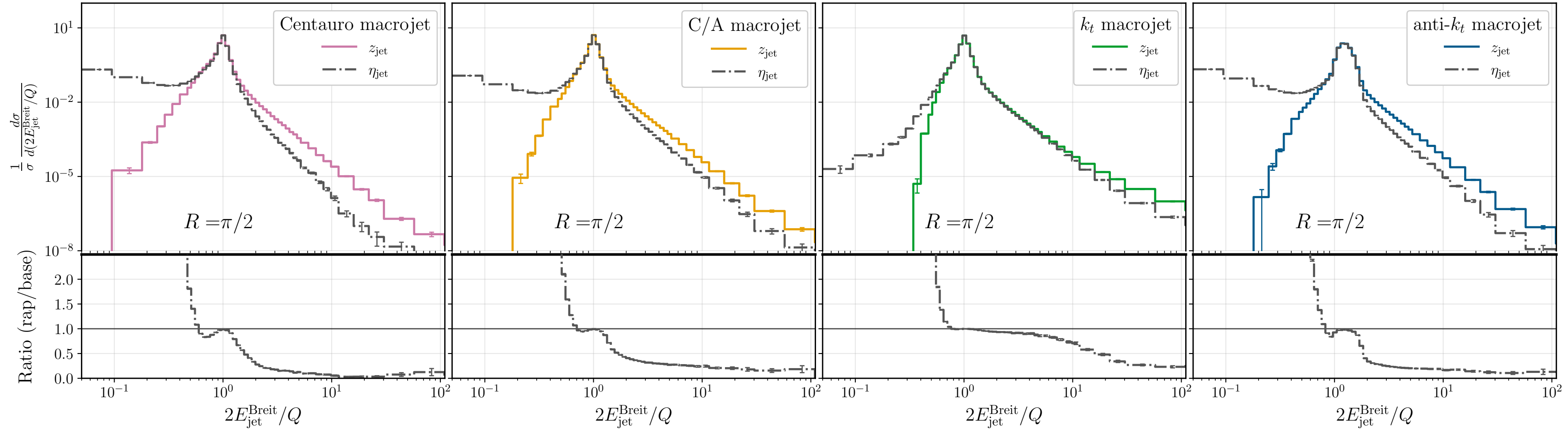
NC DIS ( ep ), \sqrt{s}=300 GeV, Q \geq 12 GeV, Macrojet reconstruction: z_{\text{jet}} vs \eta_{\text{jet}} [Pythia8(dip)]
