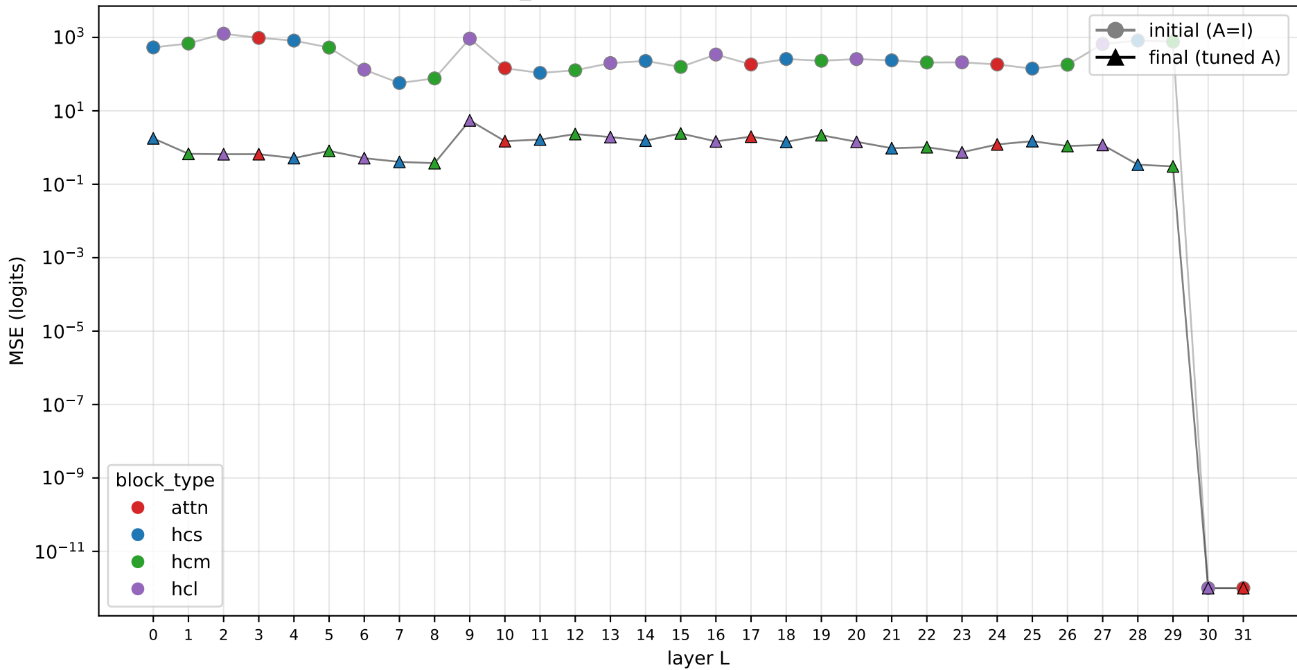
Phase 1.followup_full: tuned-lens recovery, ALL 32 layers (n=100)
