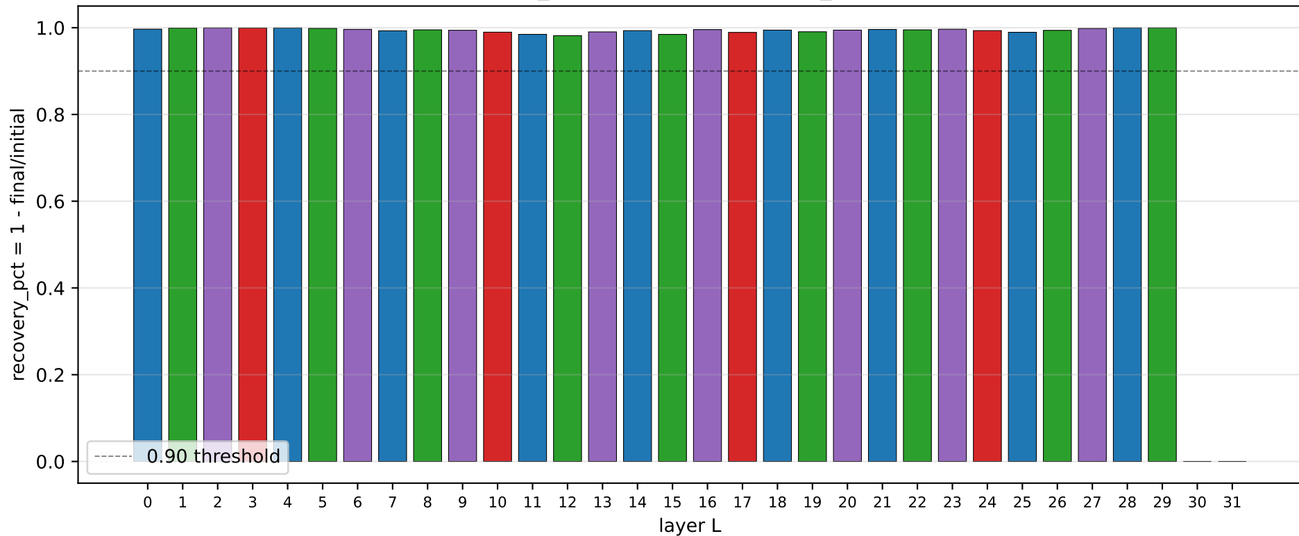
Phase 1.followup_full: tuned-lens recovery_pct, ALL 32 layers
