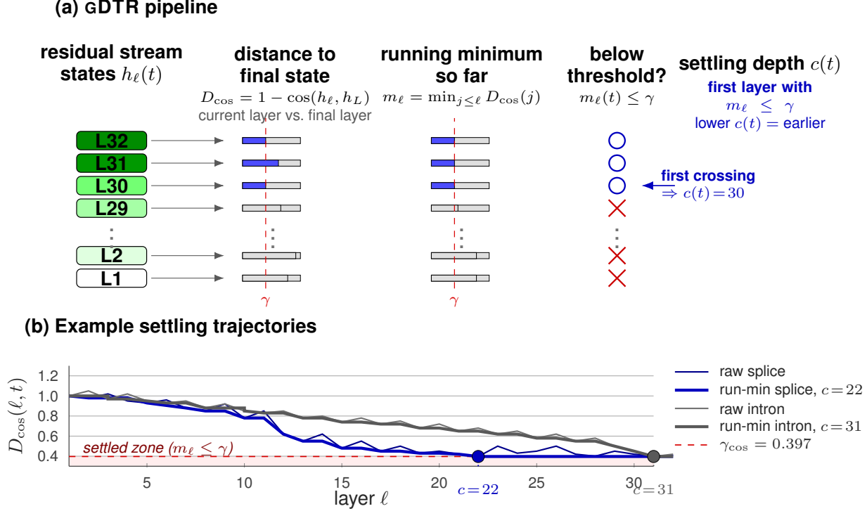
Figure 1. GDTR measures the layer at which a token’s representation stabilises. (a) Pipeline: each Evo 2 layer emits a residual-stream tap h_\ell(t) ; the cosine lens compares that tap to the final-layer state h_L(t) ; a running-minimum envelope tracks the best match so far; and the first threshold crossing defines the settling depth c(t) . Lower c(t) means earlier stabilisation. (b) Two chr22 example trajectories. Both are flat near 1 for the first \sim 5 –10 layers (representations are uninformed about the final-layer state), then descend as deeper layers commit to the post-norm direction. The splice-donor running-min (blue) crosses \gamma_{\cos} = 0.397 at \ell = 22 ; the intronic running-min (grey) crosses only at \ell = 31 . Faint traces are the raw D_{\cos}(\ell, t) ; thick traces are the running-minimum envelope (Eq. 2).
