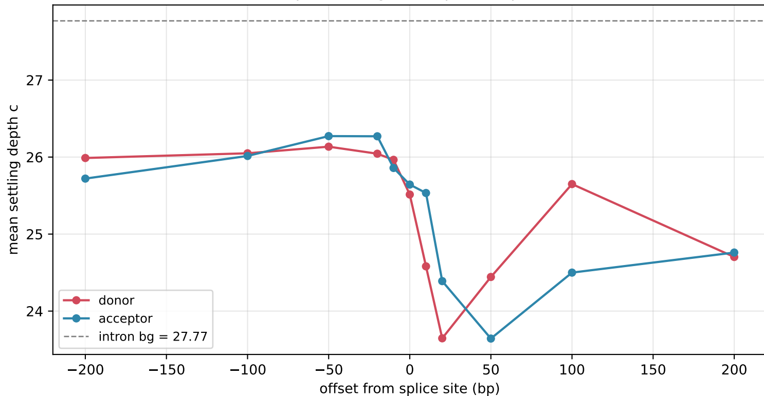
chr22 splice fine-grained profile ( \gamma=0.397 )
