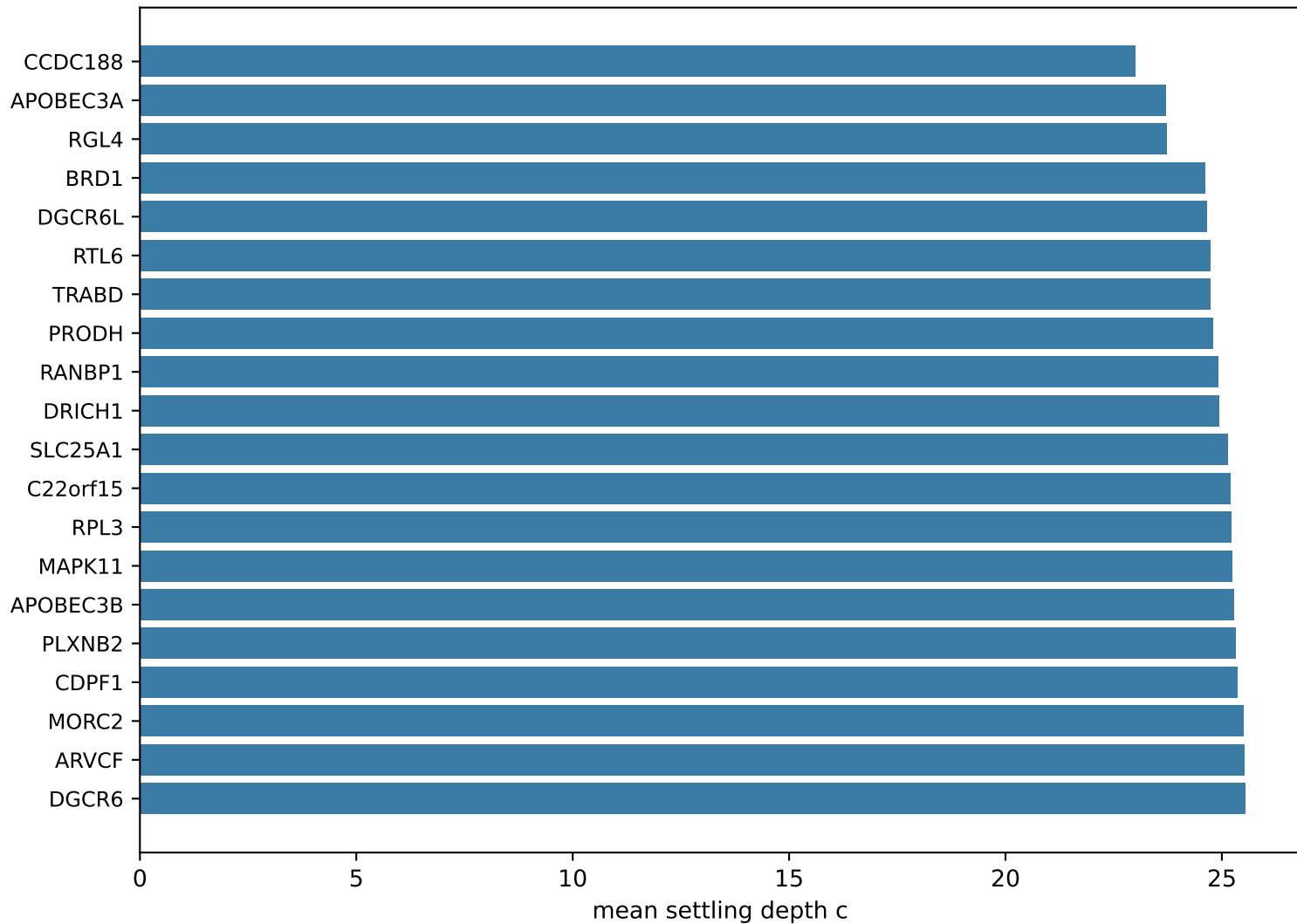
chr22 top-20 deepest-thinking genes (lowest mean c)
