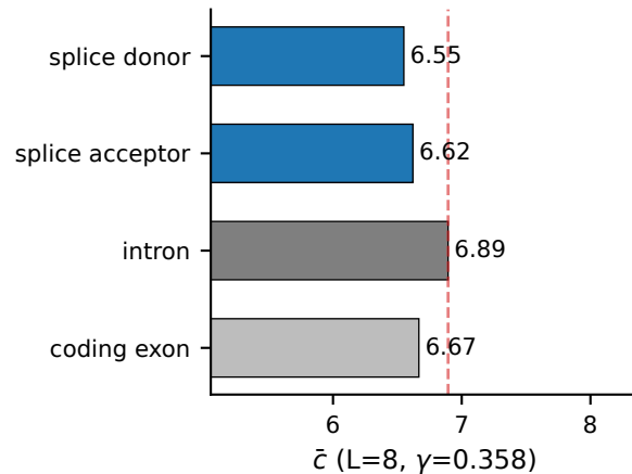
HyenaDNA-large (per-bp causal LM)
