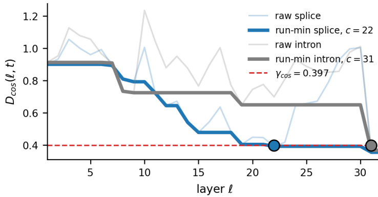
Figure 1. GDTR measures the layer at which a token’s representation stabilises. (a) Pipeline: each Evo 2 layer emits a residual-stream tap h_\ell(t) ; the cosine lens compares that tap to the final-layer state h_L(t) ; a running-minimum envelope tracks the best match so far; and the first threshold crossing defines the settling depth c(t) . Lower c(t) means earlier stabilisation. (b) Two chr22 trajectories illustrate the readout: a splice-donor token settles at \ell=22 , whereas an intronic token settles at \ell=31 .
