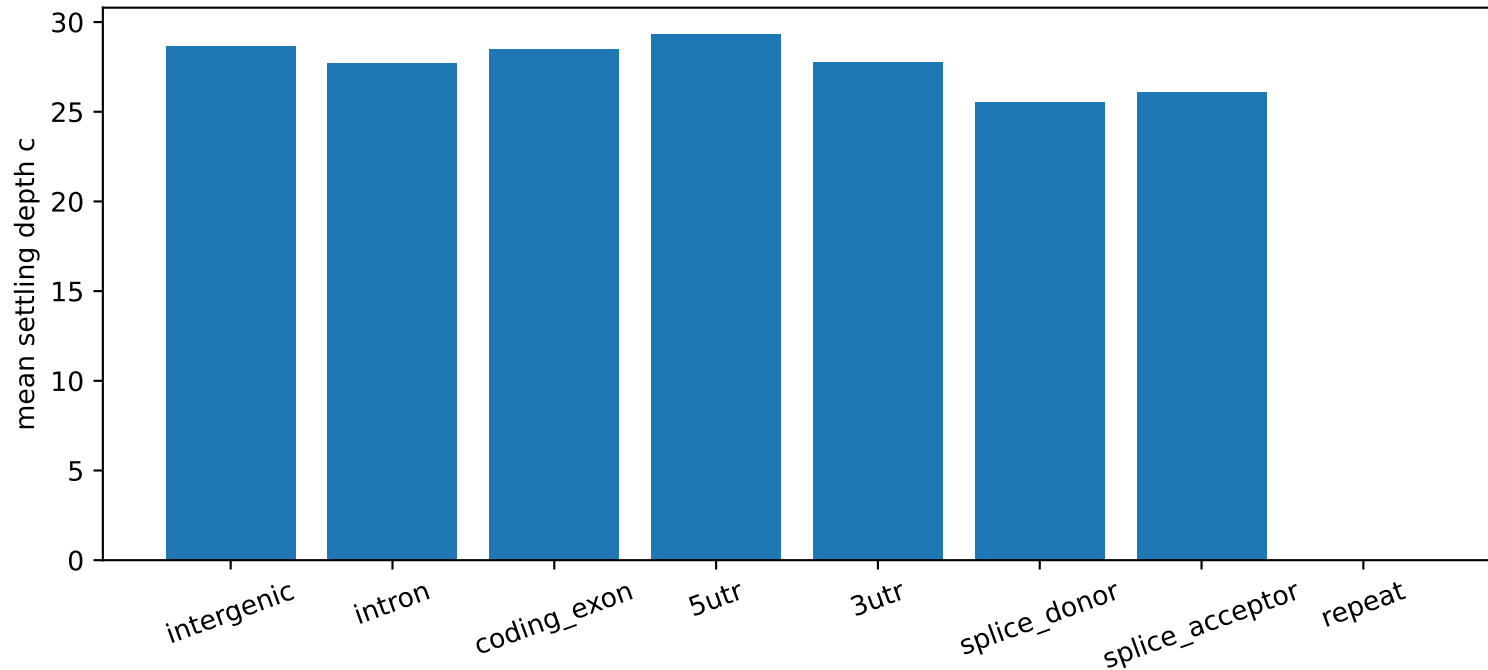
chr17 mean c per context
