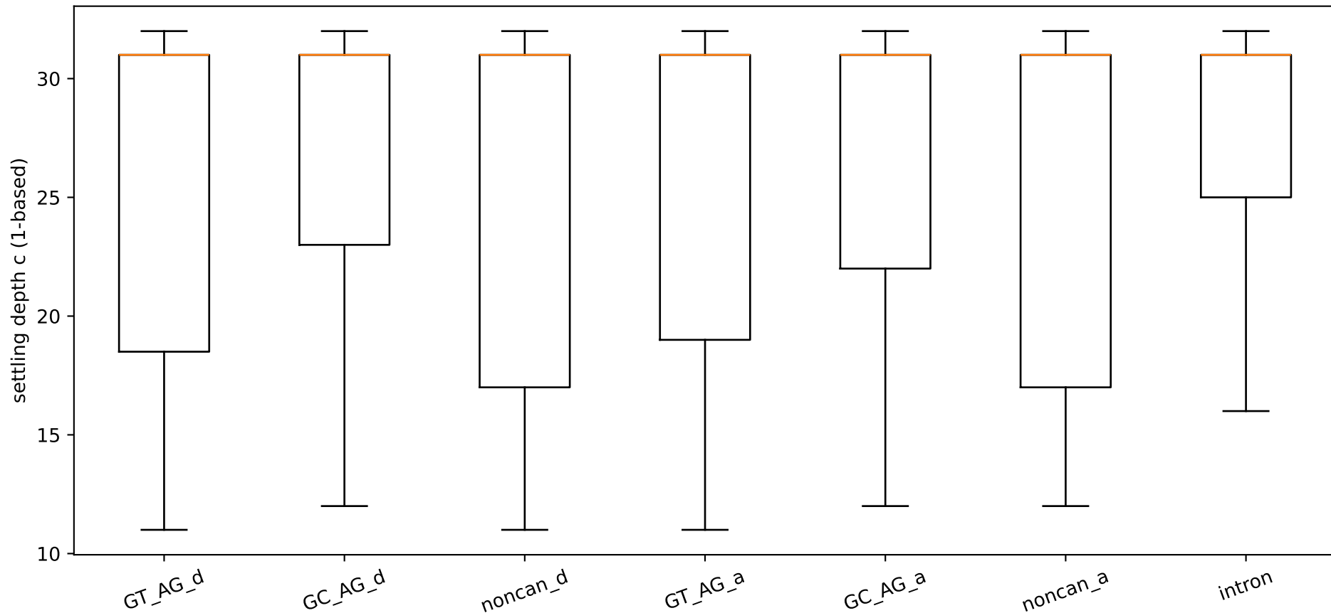
Canonical / non-canonical splice c (pooled chr17+chr22, \gamma=0.39663 )
