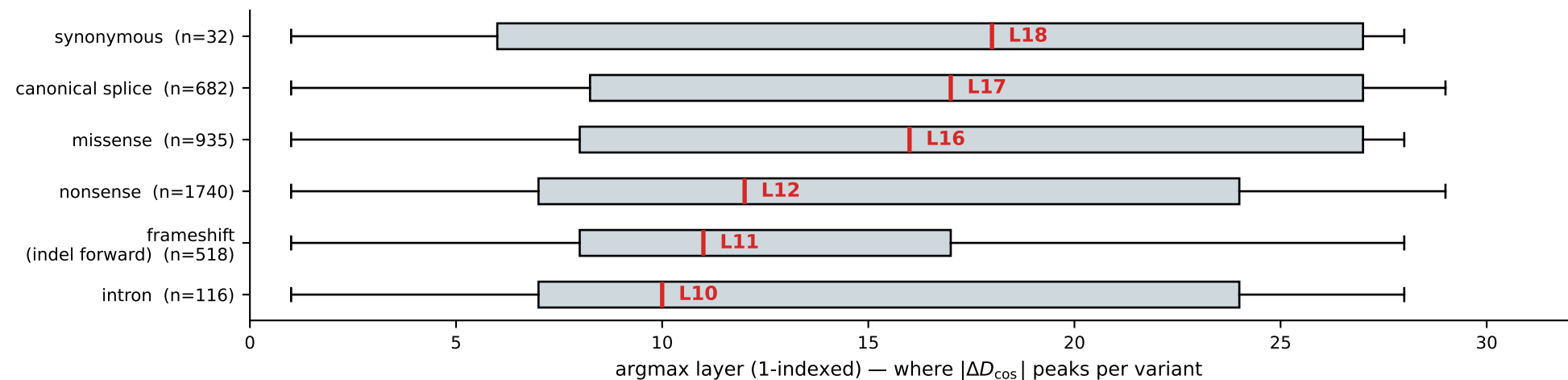
Per-class disruption layer (P/LP variants, 15 cancer-associated genes; Kruskal-Wallis 5-way p = 7.1 \times 10^{-10} )
