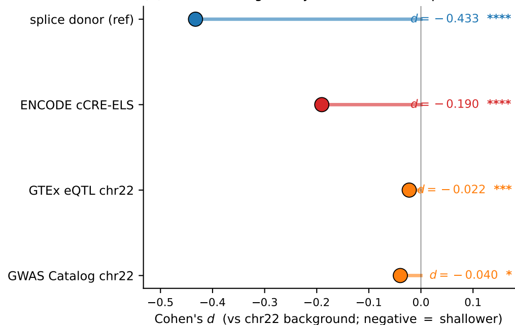
(b) Functional regulatory elements share splice shallowness axis
