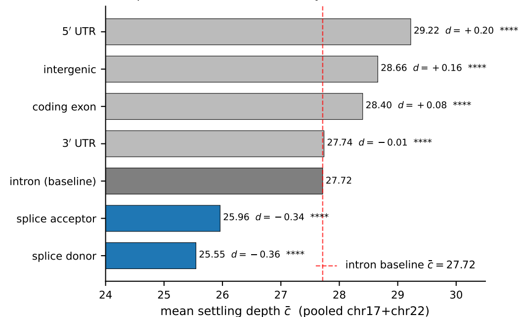
(a) Splice contexts settle ~ 2 layers shallower than introns
