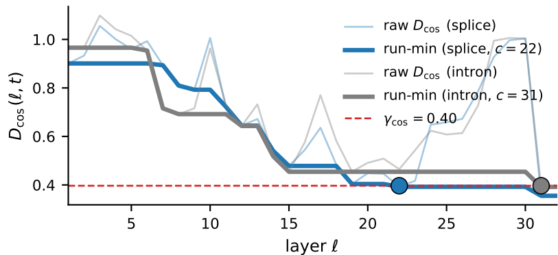
(b) Per-token settling depth on two real chr22 positions
