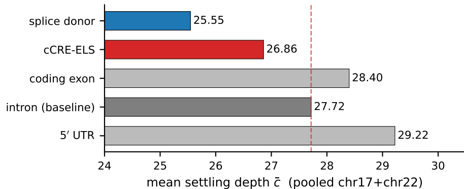
(c) Biological hierarchy of settling depth
