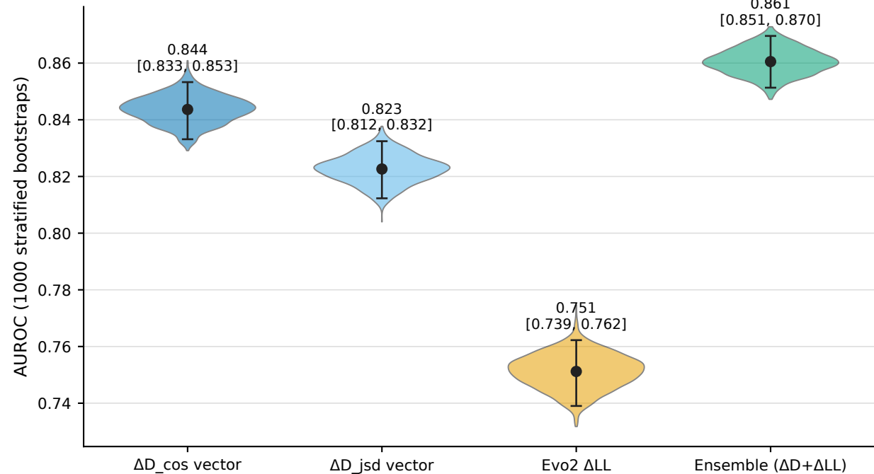
Bootstrap stability of AUROC across models
