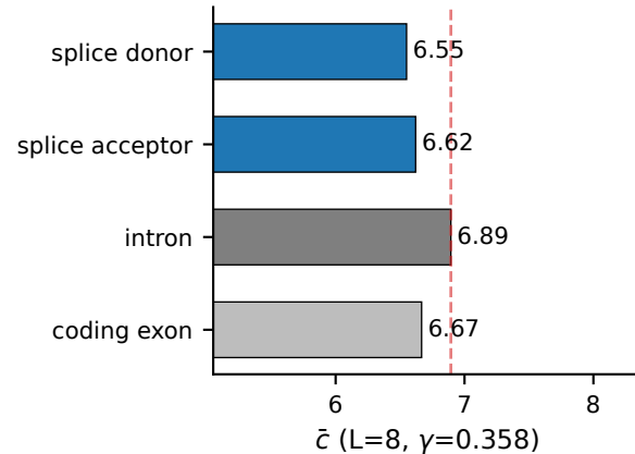
HyenaDNA-large (per-bp causal LM)
