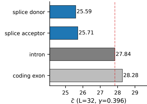
Evo 2 7B (per-bp causal LM)
