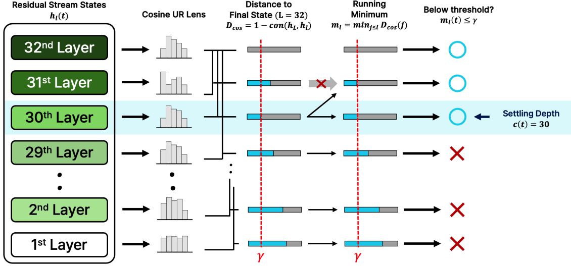
Figure 1. GDTR measures the layer at which a token’s representation stabilises. From left to right: each Evo 2 layer emits a residual-stream tap h_\ell(t) ; the cosine lens compares that tap to the final-layer state h_L (with L = 32 for Evo 2 7B) via D_{\cos}(\ell) = 1 - \cos(h_L, h_\ell) ; the running-minimum envelope m_\ell = \min_{j \leq \ell} D_{\cos}(j) collapses non-monotone descent into a monotone-non-increasing trace; and the first layer at which m_\ell falls below the calibrated threshold \gamma defines the settling depth c(t) (Eq. 2). The worked example shows a token that settles at c(t) = 30 : layer 31 alone has a larger D_{\cos} , but the running minimum carries the smaller value from layer 30 forward (the crossed-out arrow marks where the envelope refuses to increase), so m_{30} \leq \gamma is the first below-threshold layer. Earlier layers ( \ell < 30 ) and the post-norm-coupled deepest taps remain above \gamma ; lower c(t) means earlier stabilisation.
