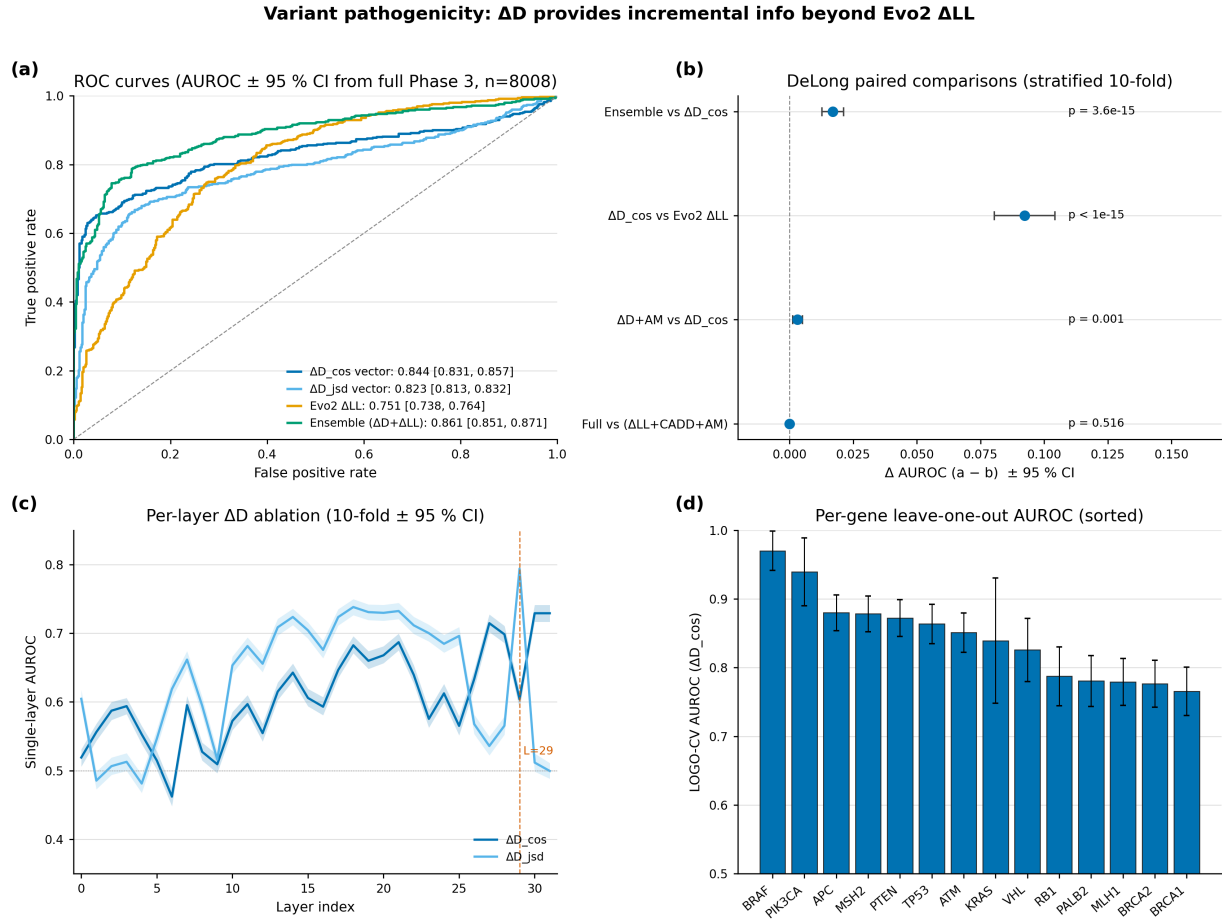
Figure 6. Variant pathogenicity discrimination on 8,008 ClinVar P/LP vs B/LB SNVs across 15 cancer-associated genes (numerical summary in Table 9). (a) ROC curves for the four scoring features. (b) Paired DeLong tests: \Delta D adds significant information beyond Evo2 \Delta LL ( p = 3.6 \times 10^{-15} ). (c) Per-layer single-feature AUROC across all 32 layers – best single tap is \ell = 29 for JSD and \ell = 30 for cosine (the latter is the post-norm rotation block, not the canonical interpretive tap; see App. A.1); the 32-d vector beats either by +0.05 to +0.12. (d) Leave-one-gene-out AUROC across 14 evaluable genes is uniformly high ( \geq 0.77 ).
