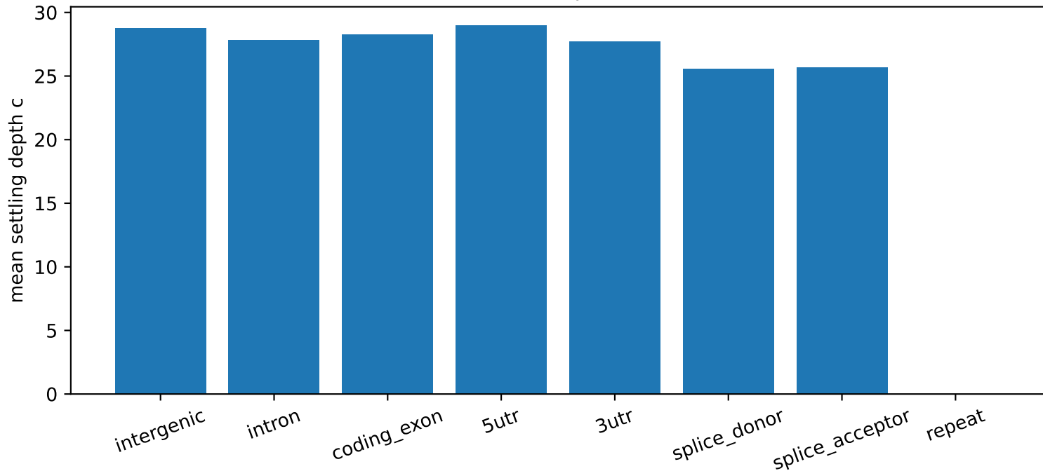
chr22 mean c per context
