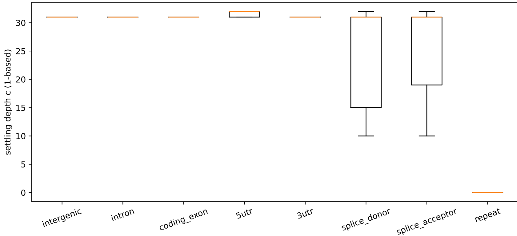
Phase 1.6 chr22 Gate B (gamma=0.397)
