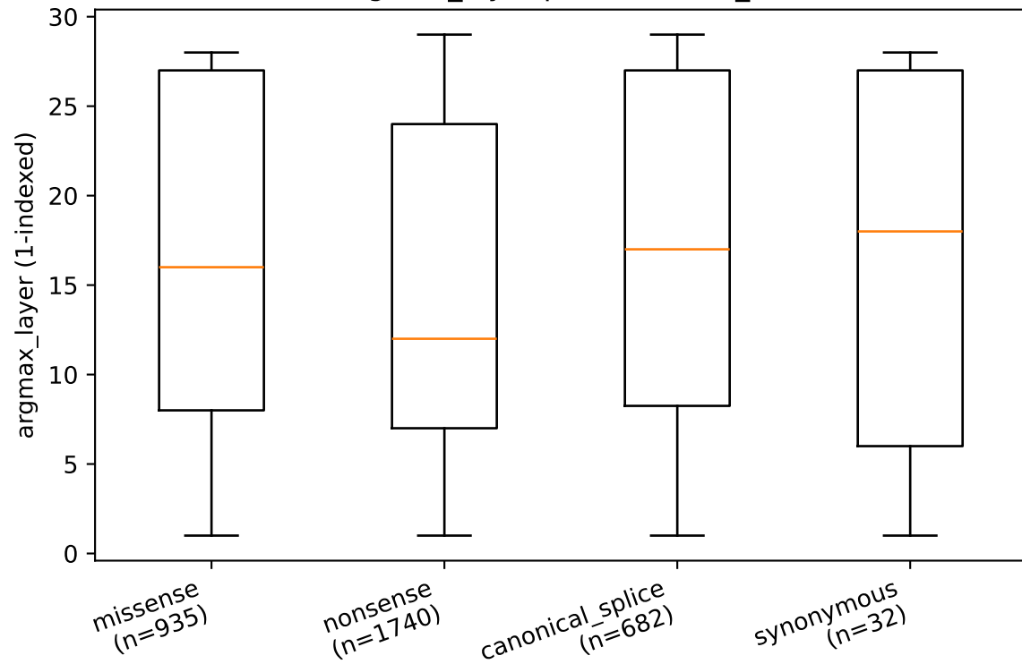
argmax_layer per class — P_LP
