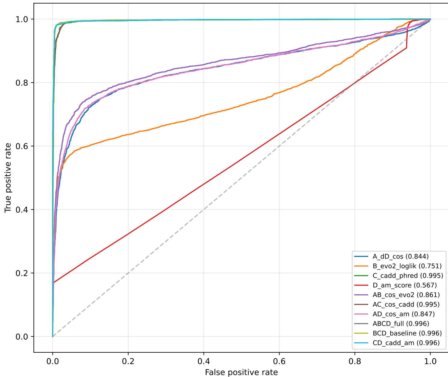
Phase 3 ensemble ROC — stratified 10-fold (n=8008)
