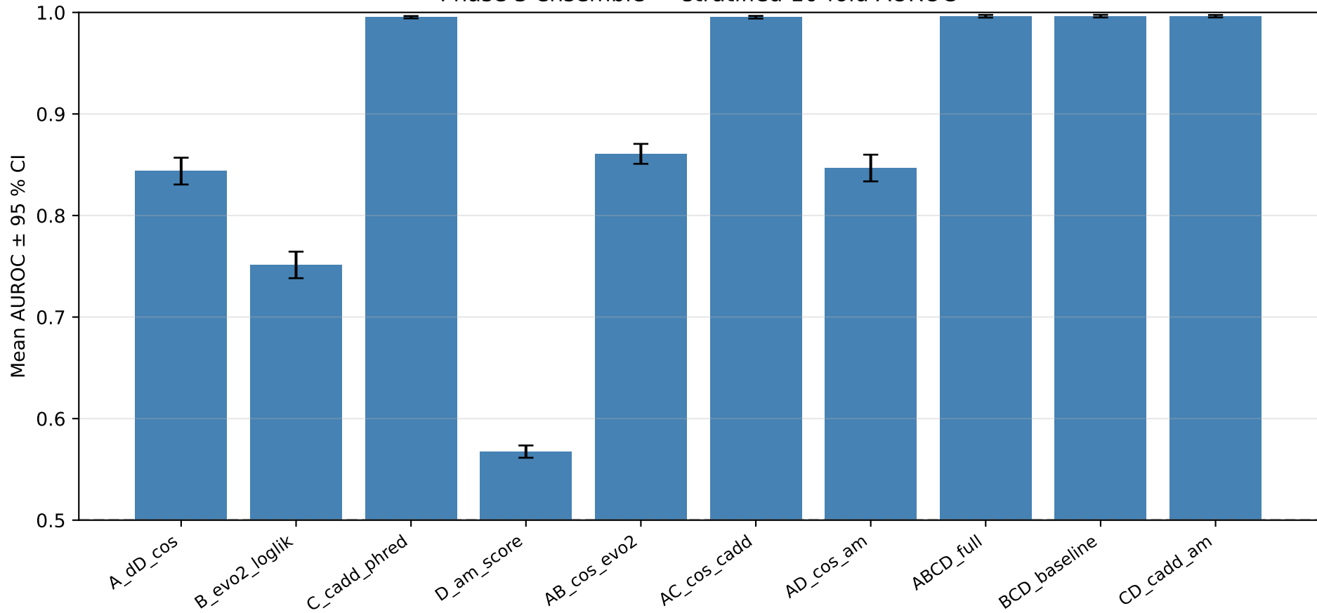
Phase 3 ensemble — stratified 10-fold AUROC
