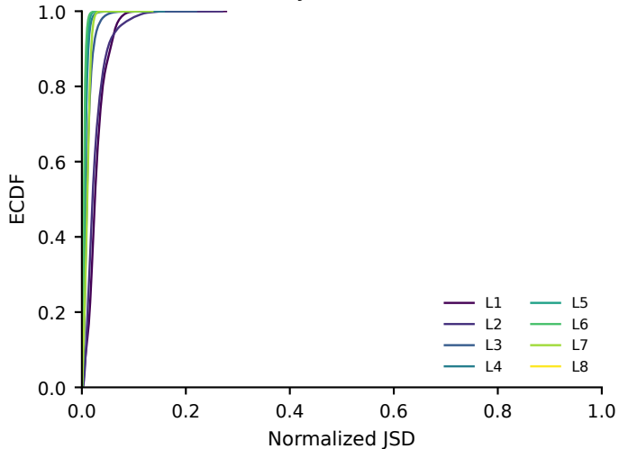
(b) Per-layer ECDF (viridis)
