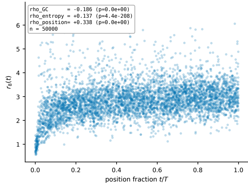
D5 - Position-stratified r_8
