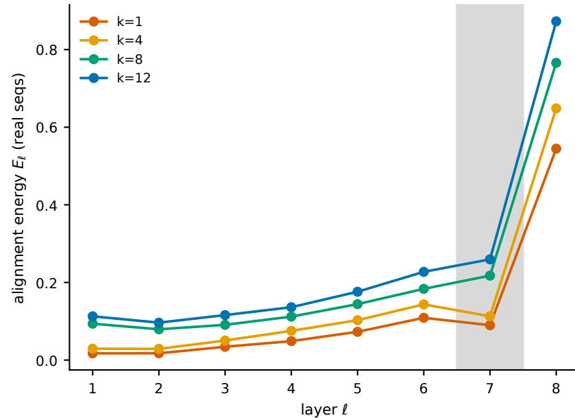
D4 - Im_head SVD alignment by layer
