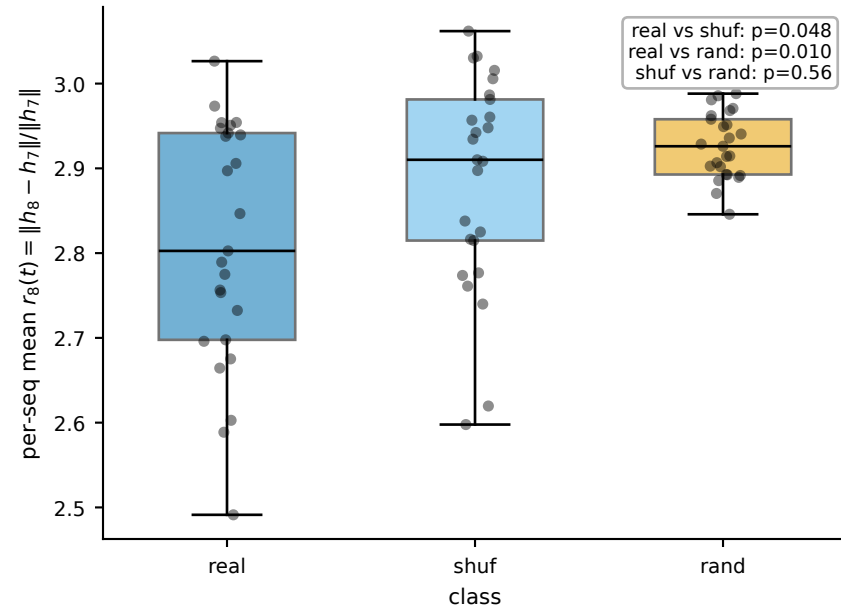
D3 - Block-8 relative residual norm
