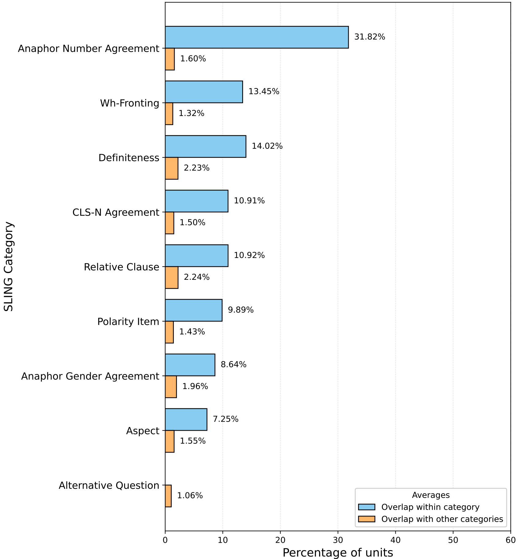
Cross-phenomenon overlap in SLING (gemma-3-4b-pt)
