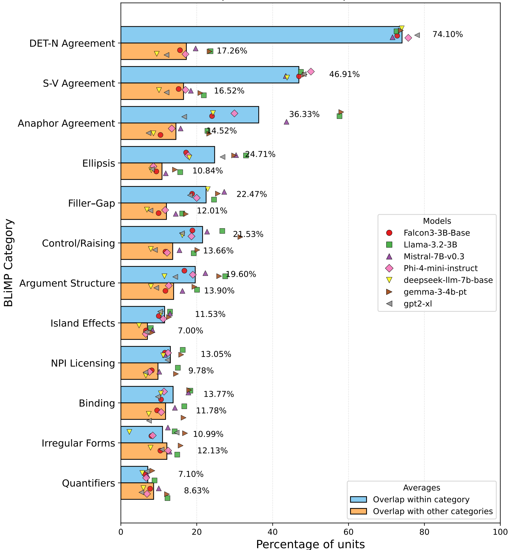
Cross-phenomenon overlap in BLiMP (5%)
