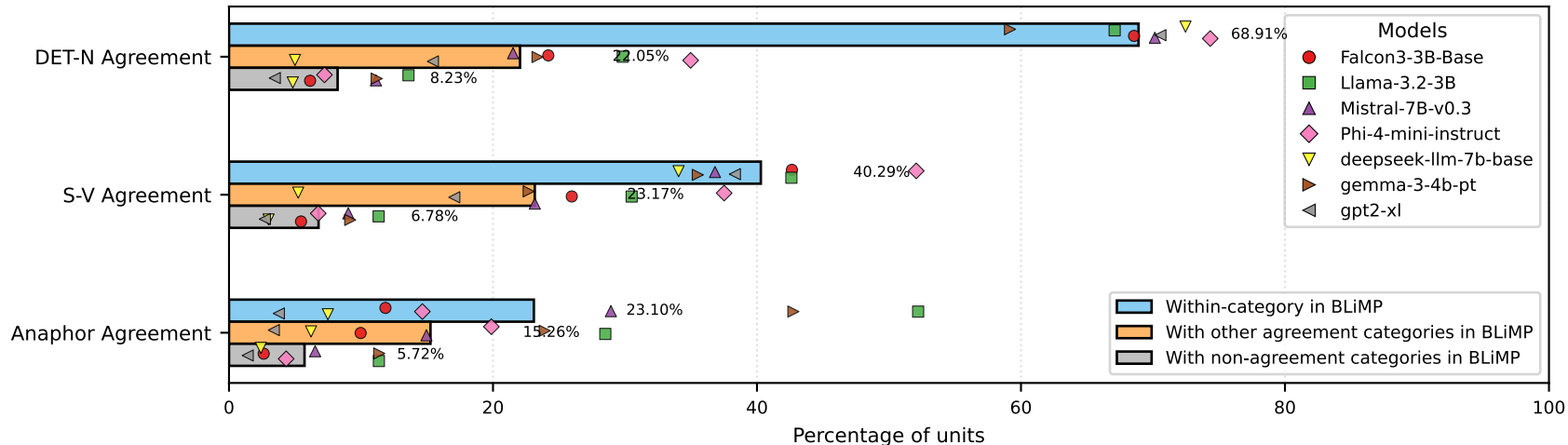
Cross-phenomenon overlap in BLiMP (agreement)
