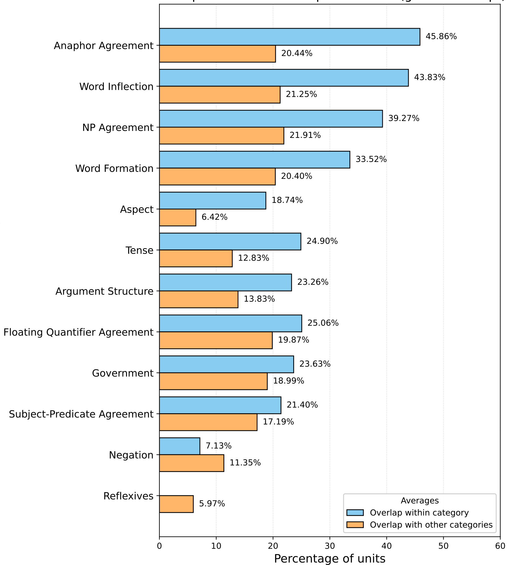
Cross-phenomenon overlap in RuBLiMP (gemma-3-4b-pt)
