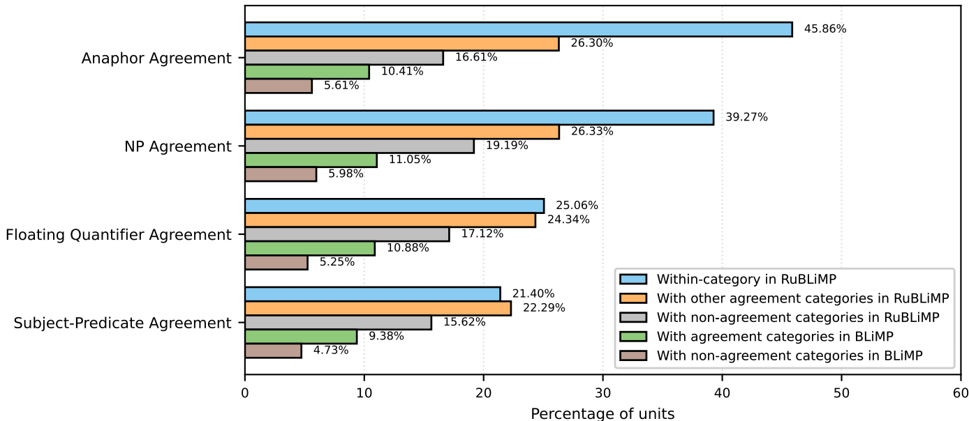
Cross-phenomenon overlap in RuBLiMP (agreement, gemma-3-4b-pt)
