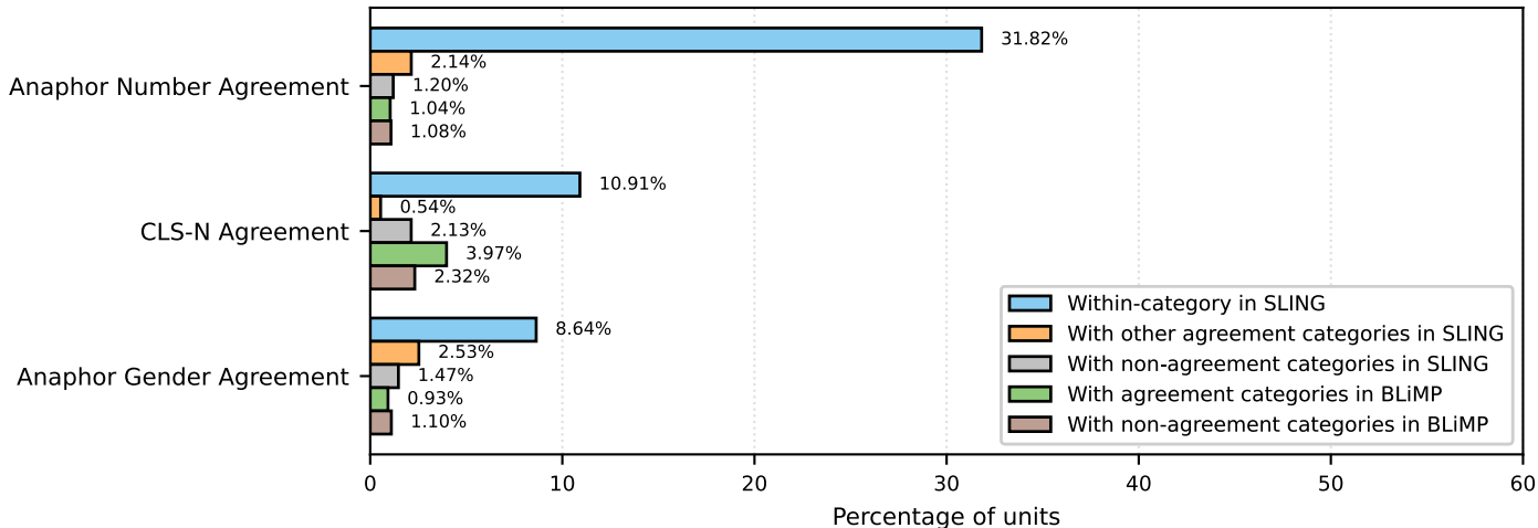
Cross-phenomenon overlap in SLING (agreement, gemma-3-4b-pt)
