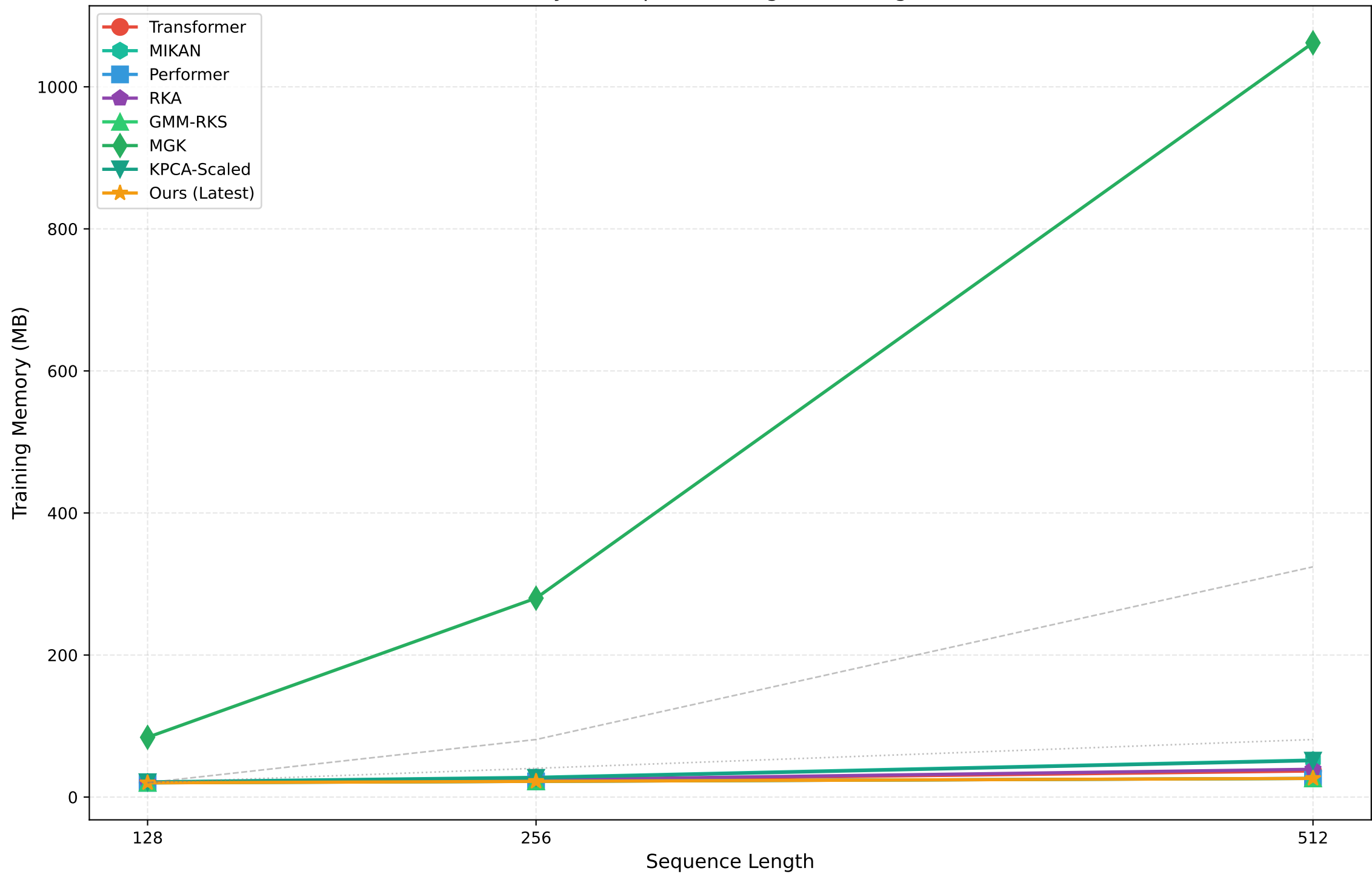
Memory vs Sequence Length (Training Mode)
