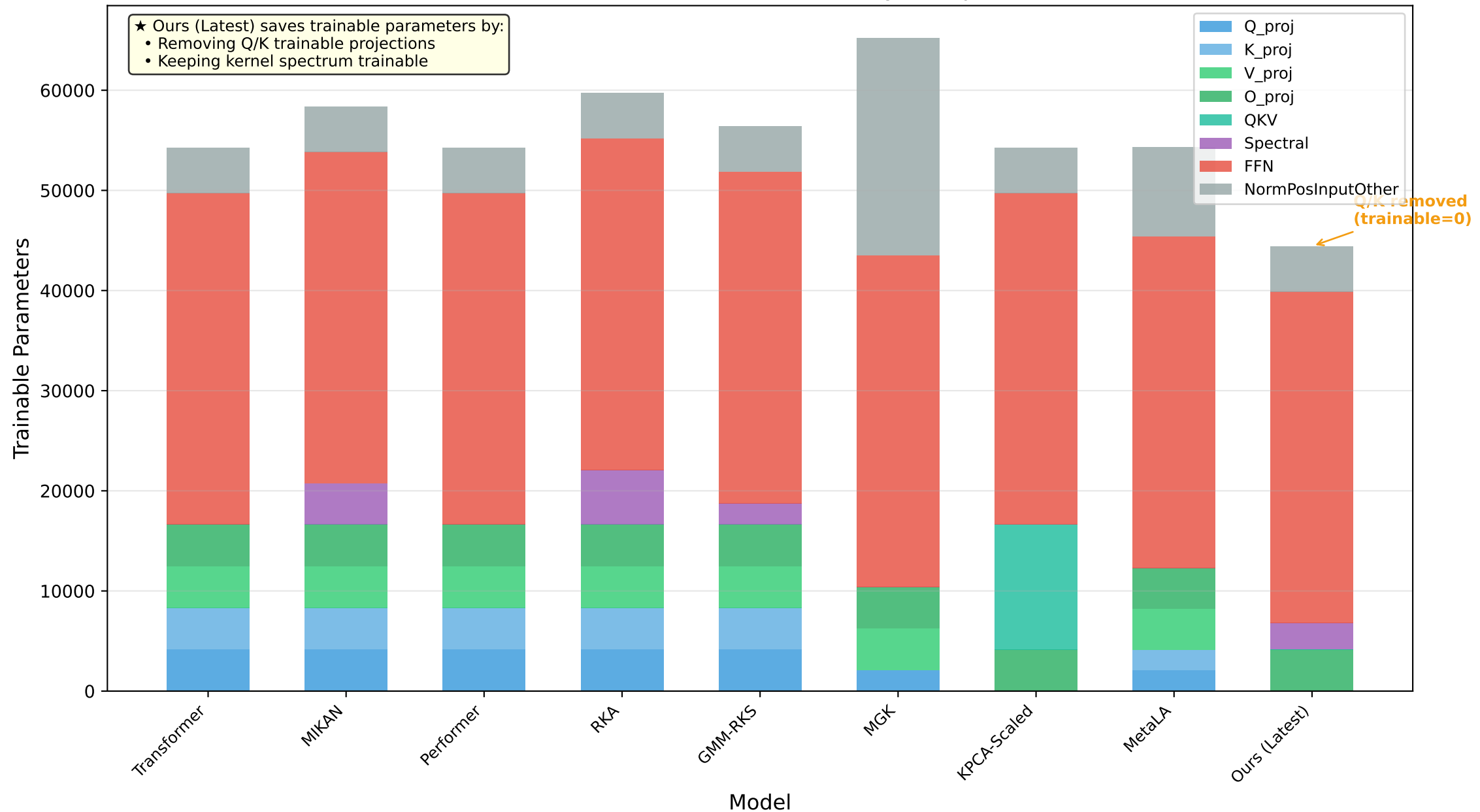
Trainable Parameter Breakdown by Component
