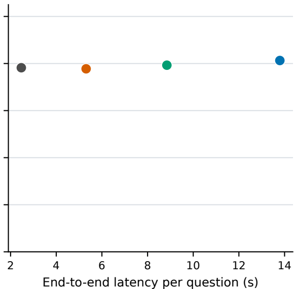
ARC-Challenge
