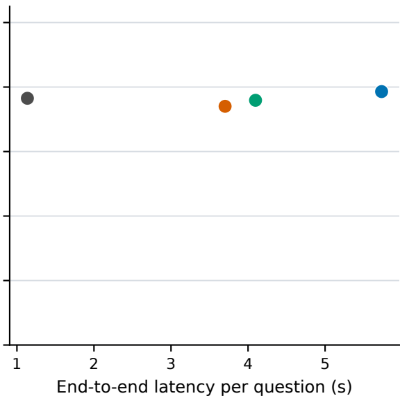
BoolQ
