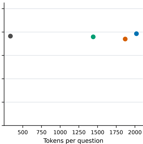
BoolQ
