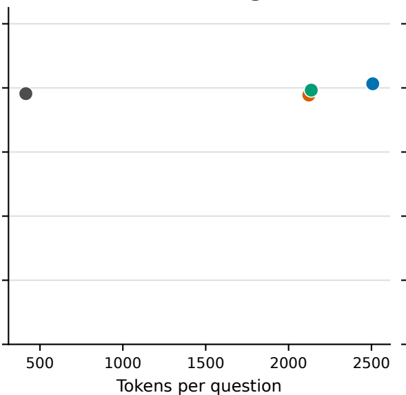
ARC-Challenge
