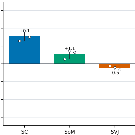
ARC-Challenge
