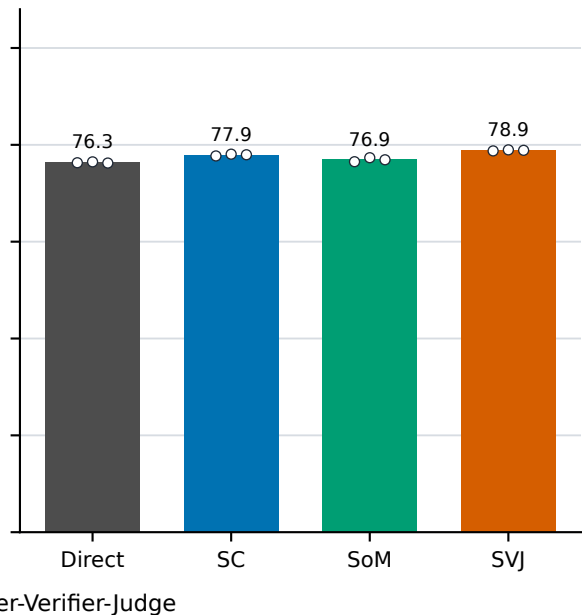
BoolQ
