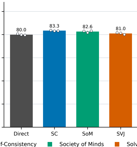
ARC-Challenge
