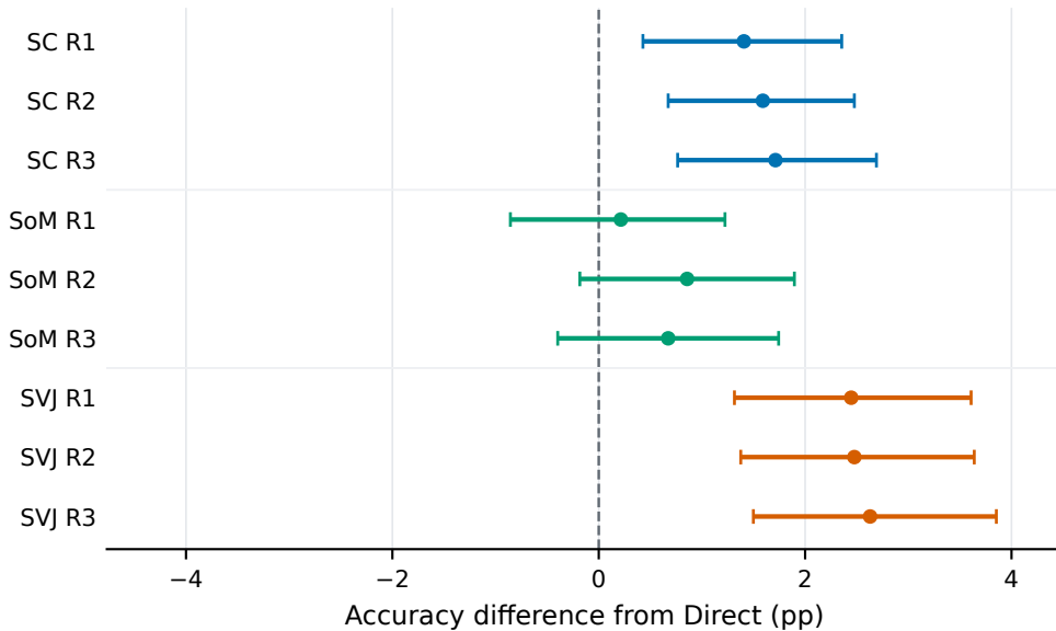
Qwen2.5-3B - BoolQ
