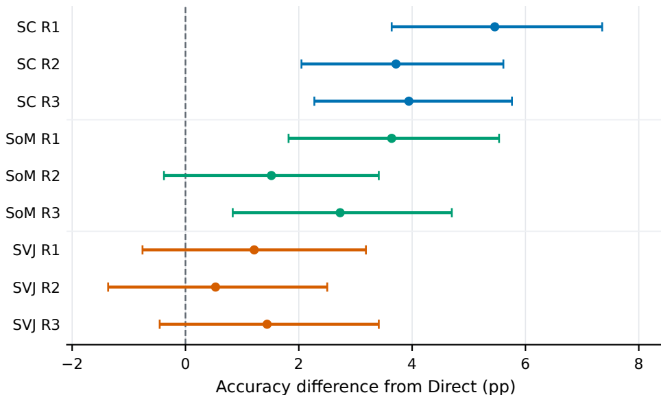
Qwen2.5-3B - ARC-Challenge
