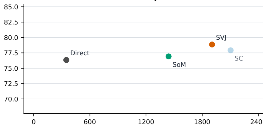
Qwen2.5-3B BoolQ
