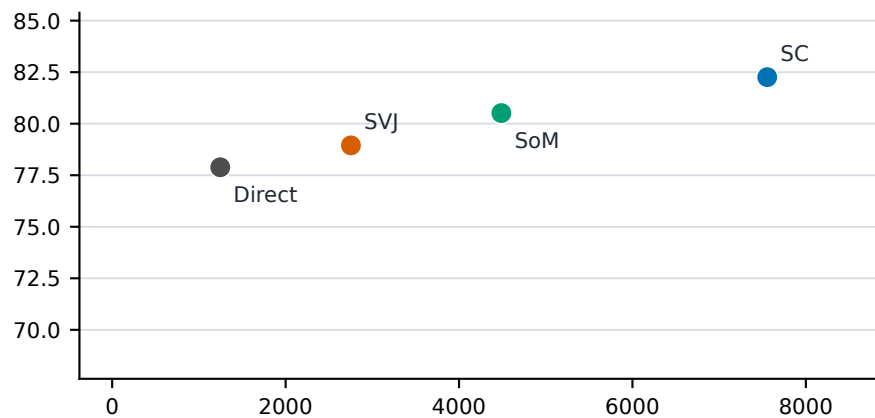
Qwen2.5-3B ARC-Challenge
