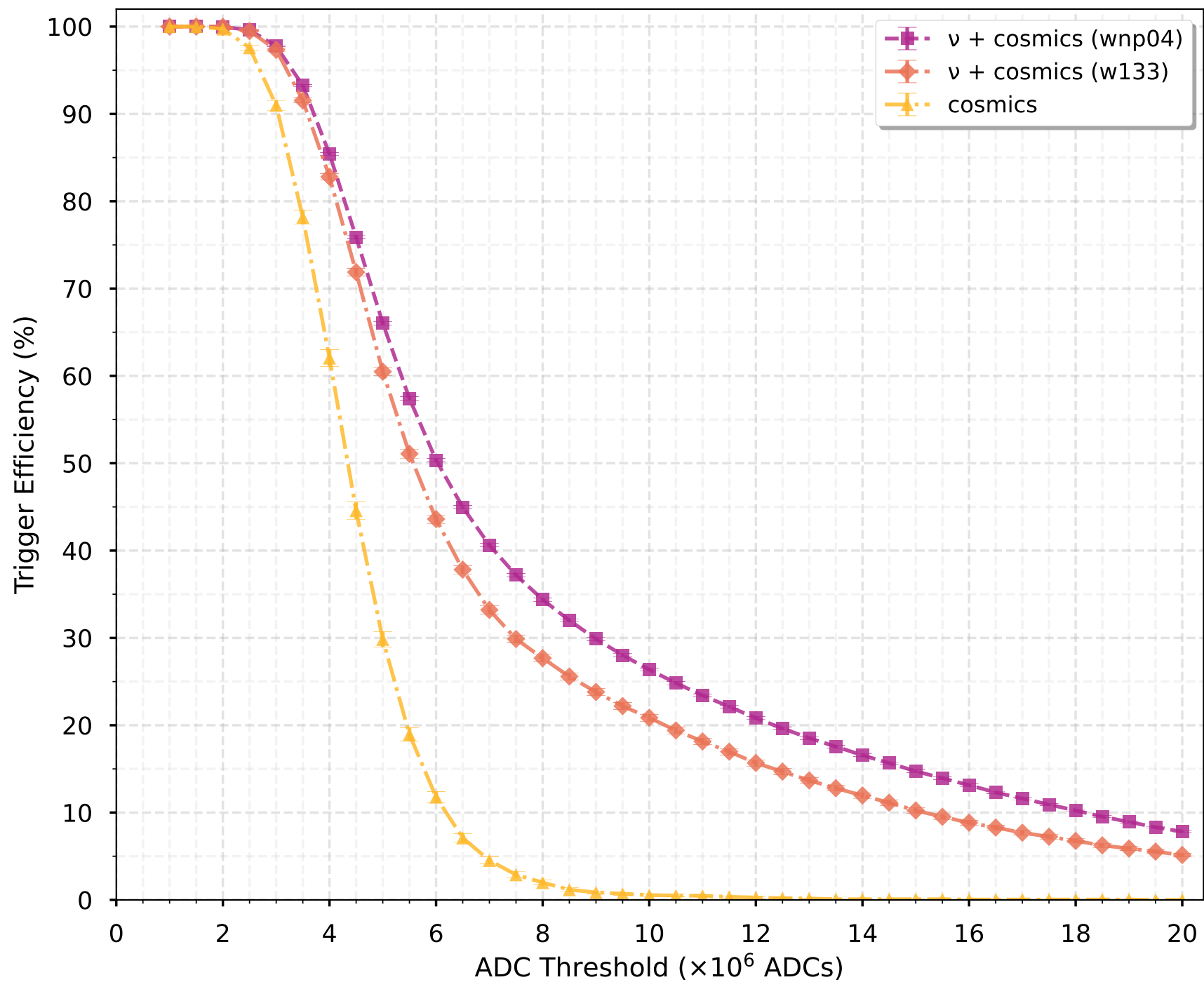
Trigger Efficiency for Neutrinos in PD-HD
