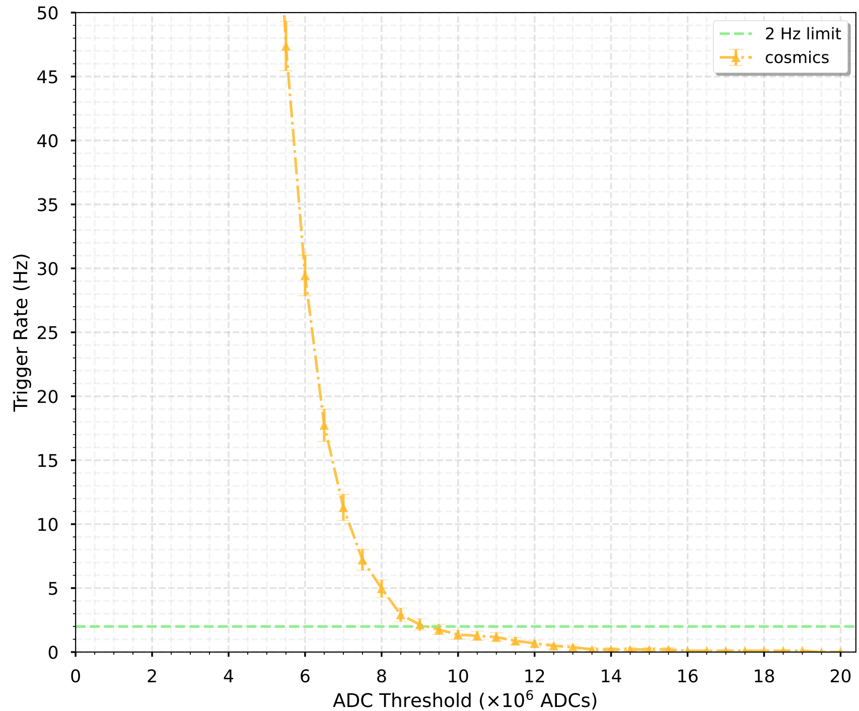
Trigger Rate for Cosmics in PD-HD
