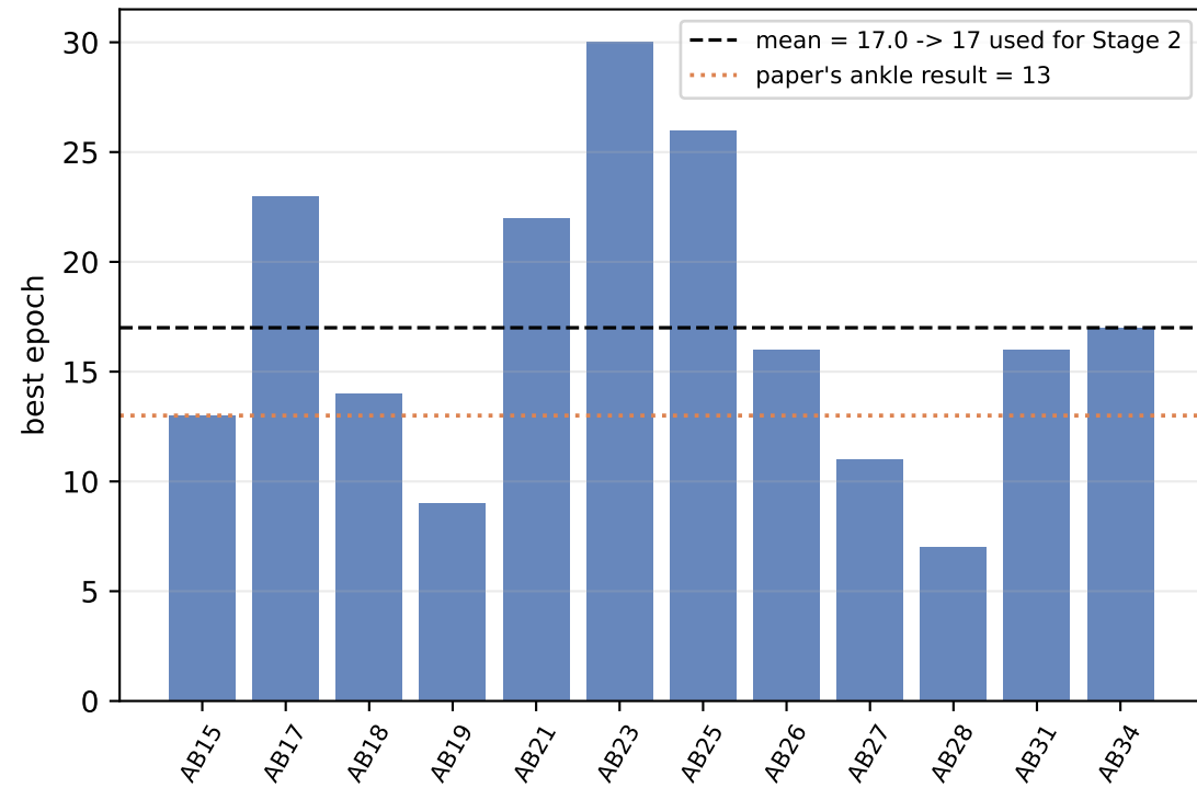
Stage 1: LOSO early-stopping epoch
