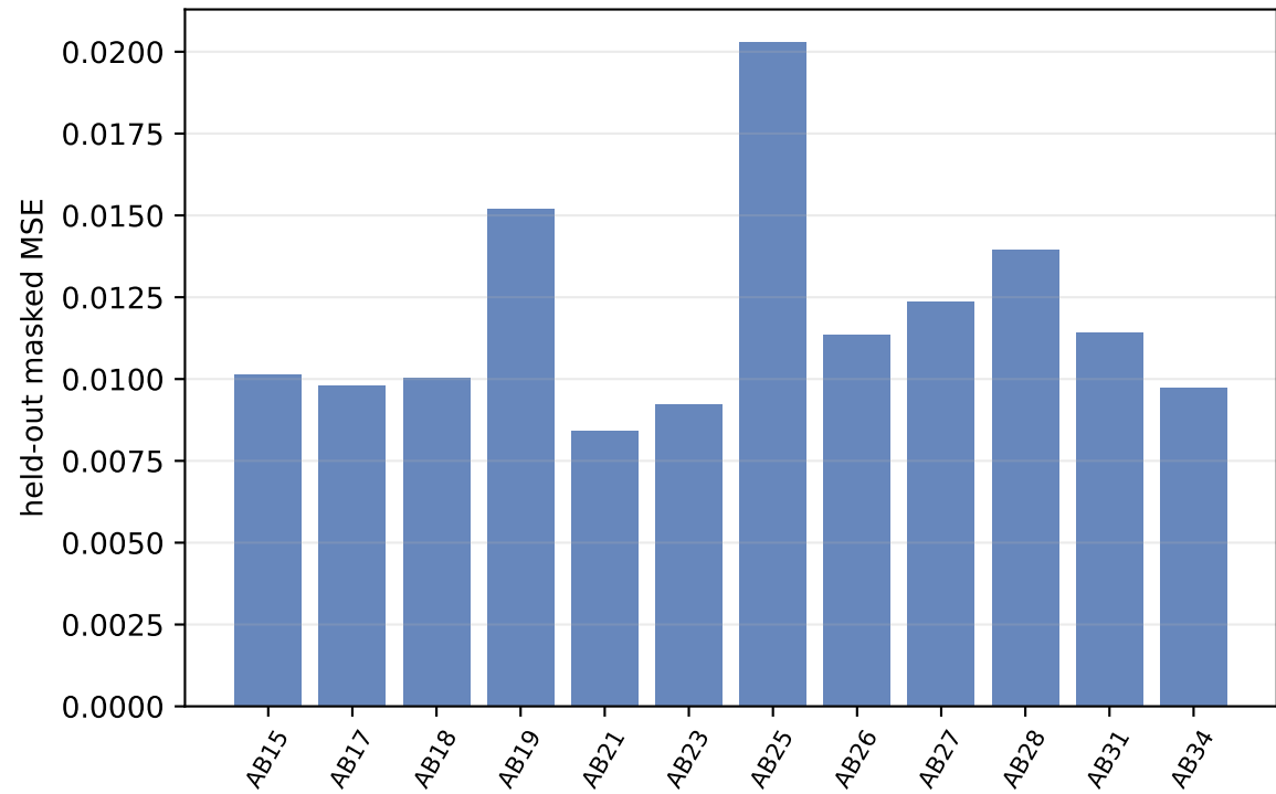
Stage 1: per-subject validation loss
