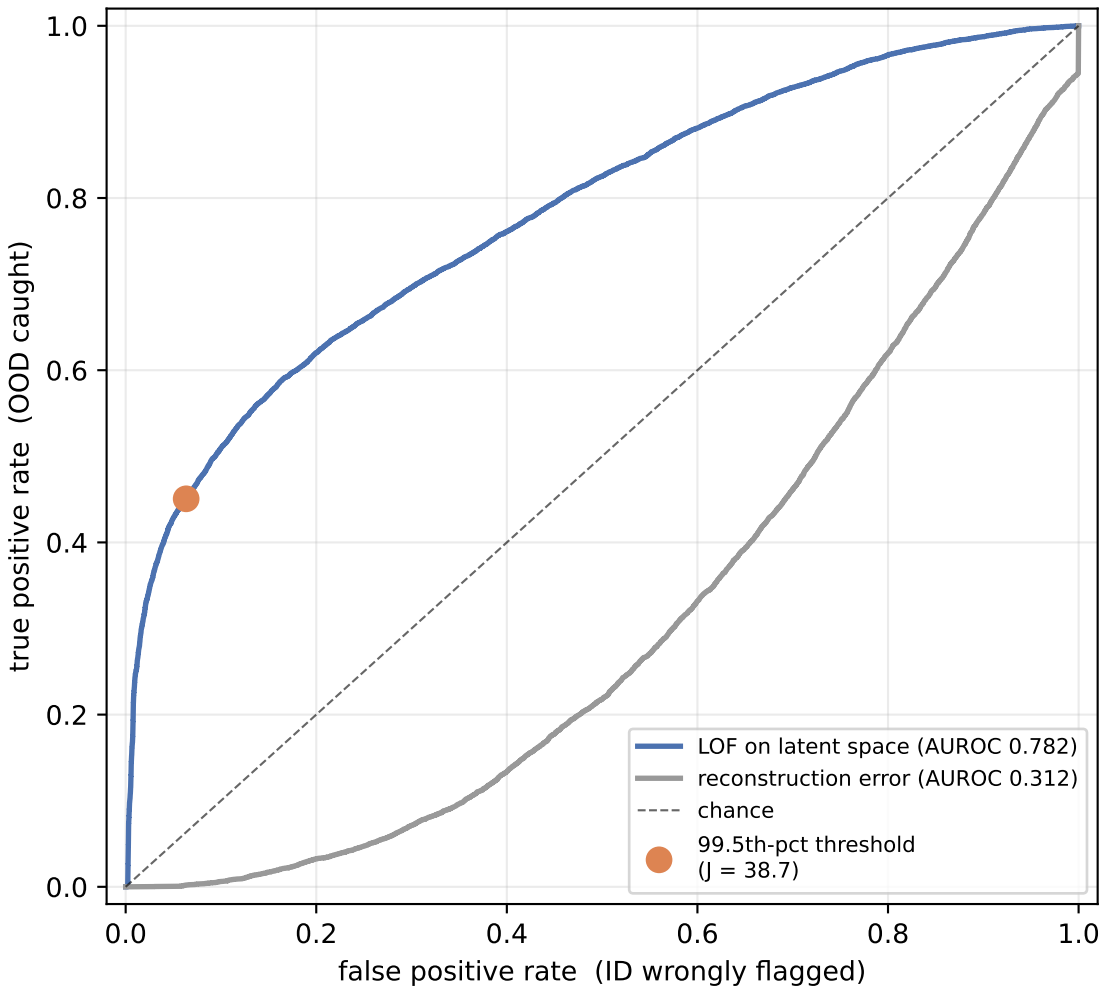
Autoencoder: ID vs held-out modes
