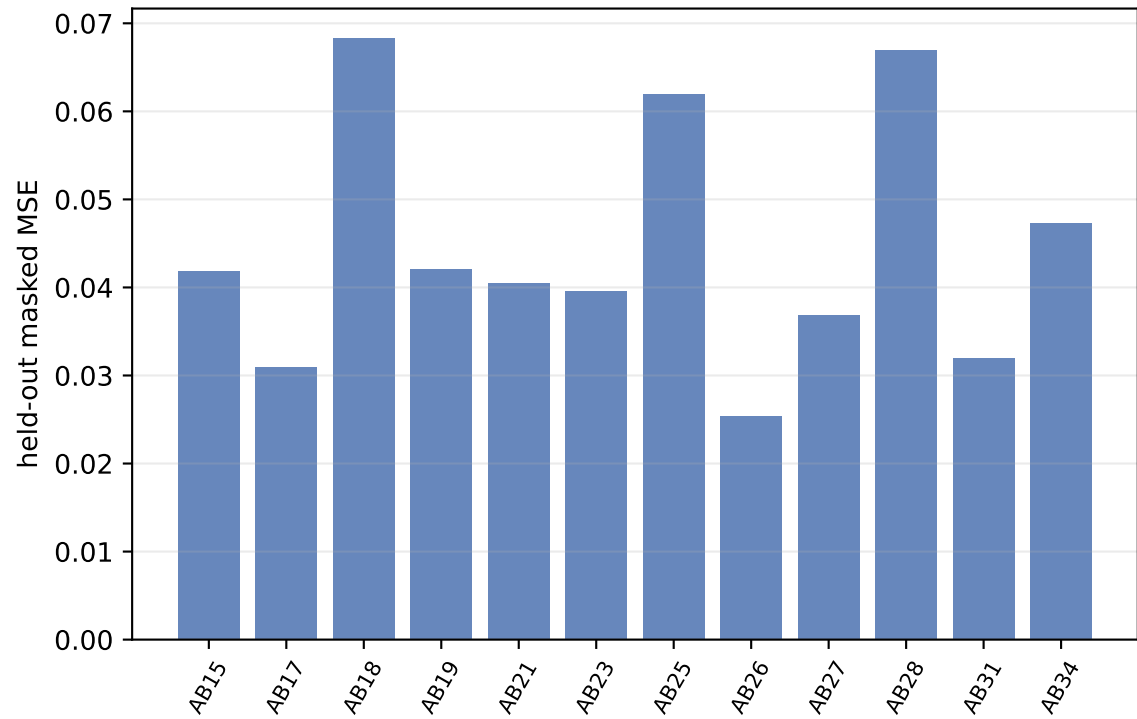
Stage 1: per-subject validation loss
