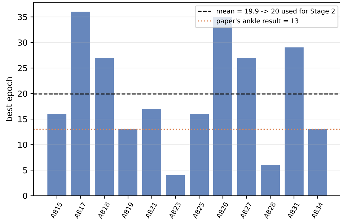
Stage 1: LOSO early-stopping epoch
