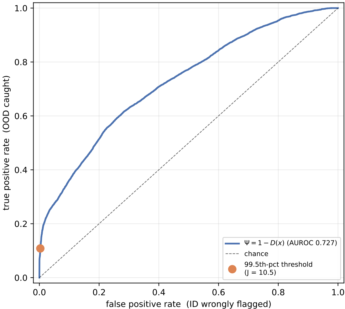
GAN discriminator: ID vs held-out modes
