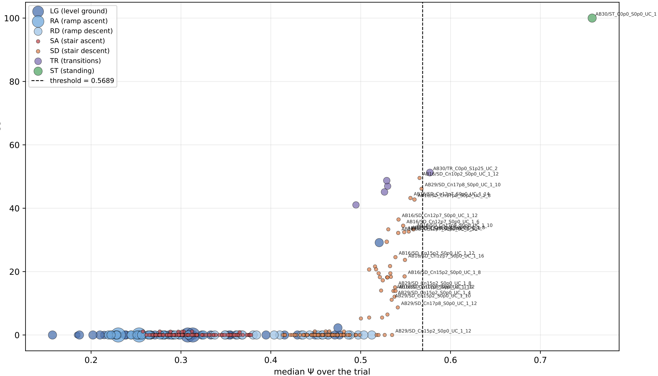
Per-trial scores — marker size is window count, labels are the 22 highest-scoring trials
