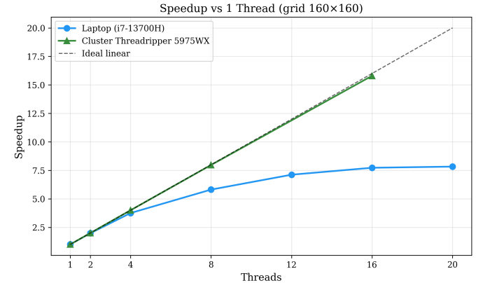
Fig. 15. OpenMP speedup versus single-thread baseline for the largest available grid size.
