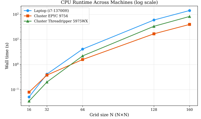
Fig. 14. Best CPU runtime across laptop and cluster machines (log scale).
