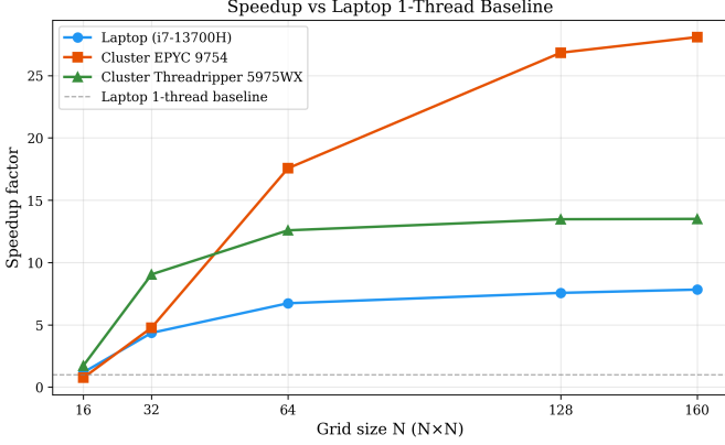
Fig. 17. Speedup of each machine relative to the laptop single-thread baseline.
