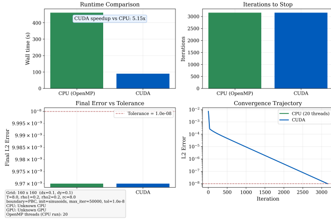
Fig. 13. Laptop convergence comparison for default physical parameters. CPU and CUDA converge to the same error threshold with identical iteration counts.
