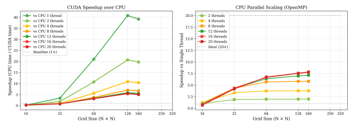
Fig. 12. Laptop benchmark speedups: CUDA over CPU (left) and CPU OpenMP scaling (right).
