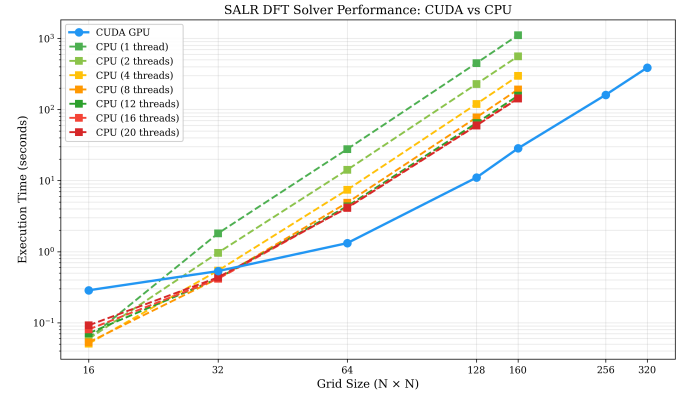
Fig. 11. Laptop benchmark runtime for CUDA and CPU across grid sizes.
