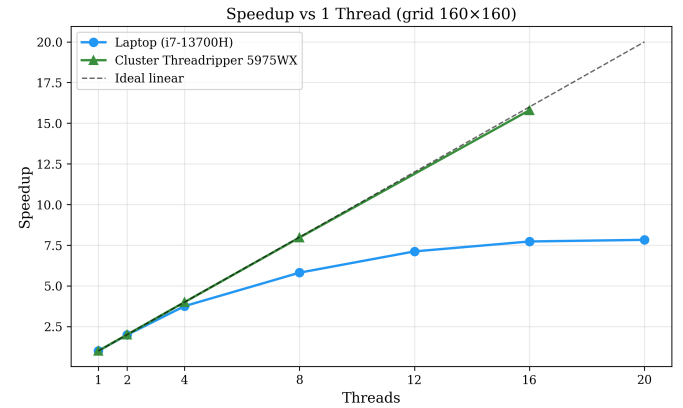
Fig. 15. OpenMP speedup versus single-thread baseline for the largest available grid size.
