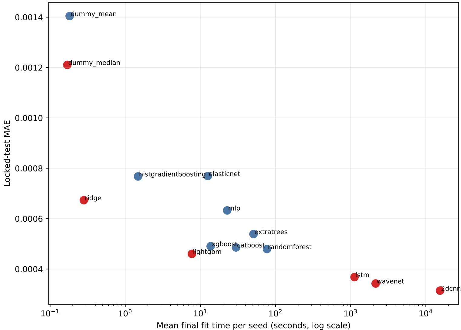
Accuracy-cost Pareto audit
