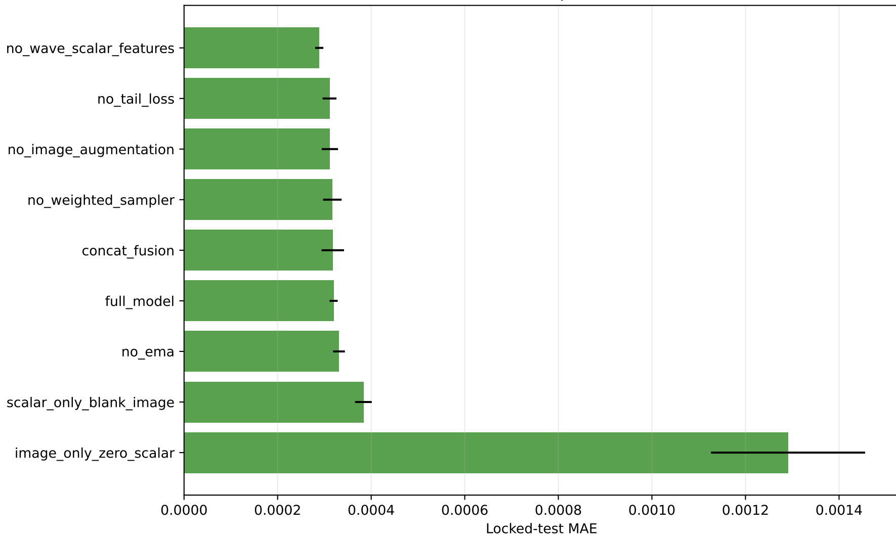
2D-CNN ablation performance
