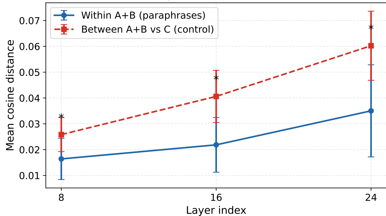
Representation convergence across layers (* = p < 0.0167 , Bonferroni)
